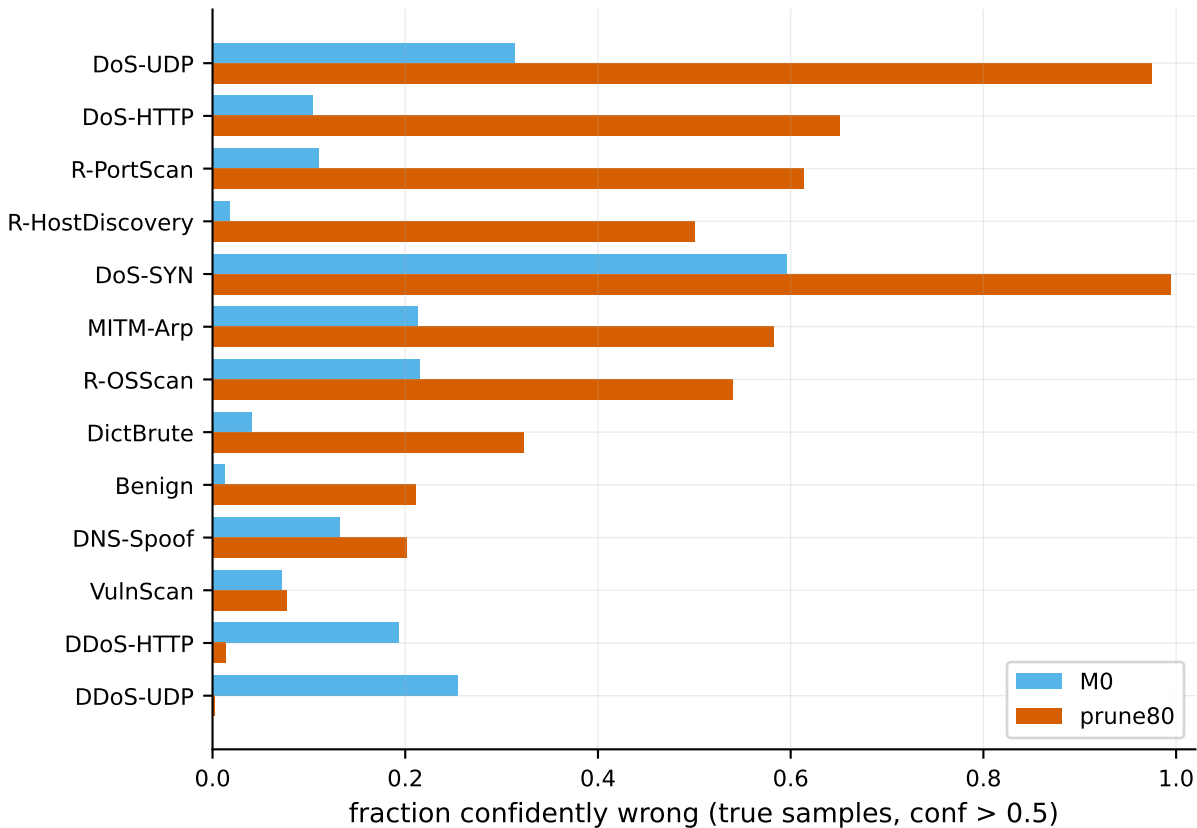
Confident-wrongness rises under prune80 (CNN, measurable classes)
