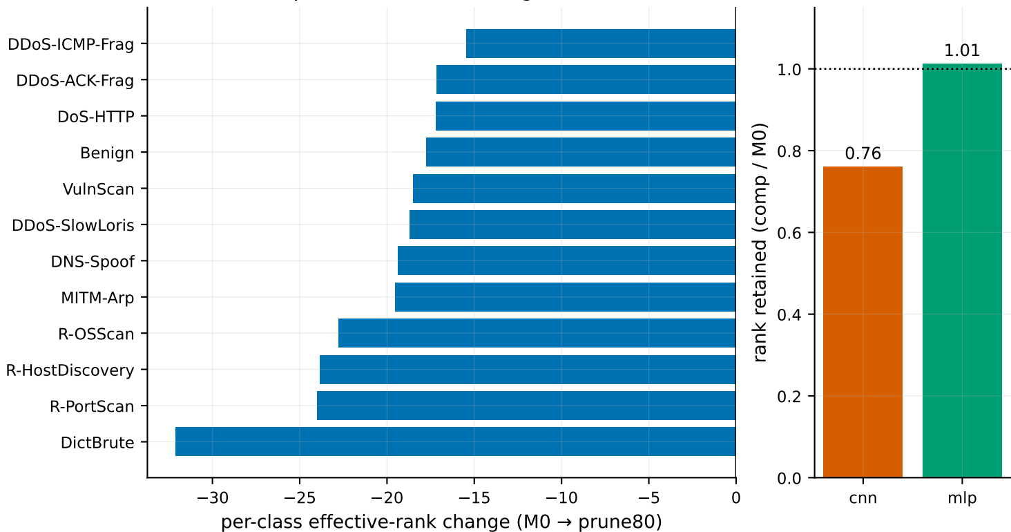
CNN per-class rank loss (largest losses)
