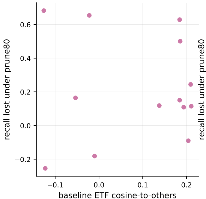
Neural-collapse geometry (Spearman vs \Delta\text{recall} = +0.19 , n.s.)
