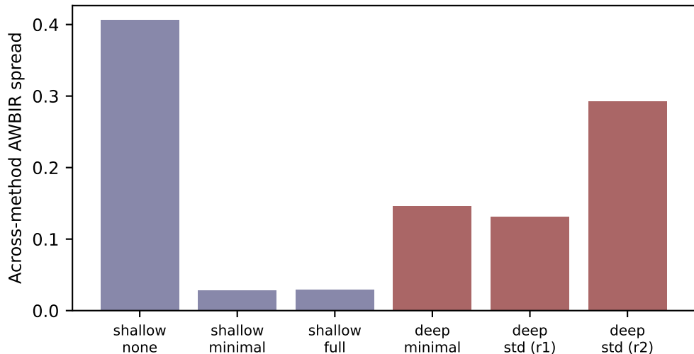
Selection-effect magnitude by regime (validation, 40%)
