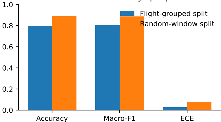
Window-level metrics by split protocol
