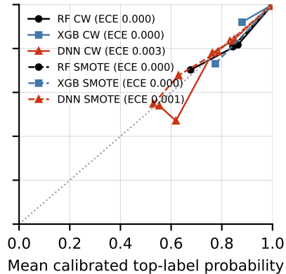
CIC-IDS2017
