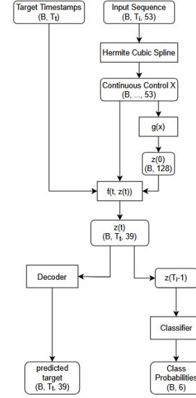
Figure 4: Workflow of the proposed method. It uses a differentiable Hermite cubic spline that can be integrated to obtain the hidden state at arbitrary timestamps. The final hidden state is used to obtain class probabilities, similar to RNNs.
