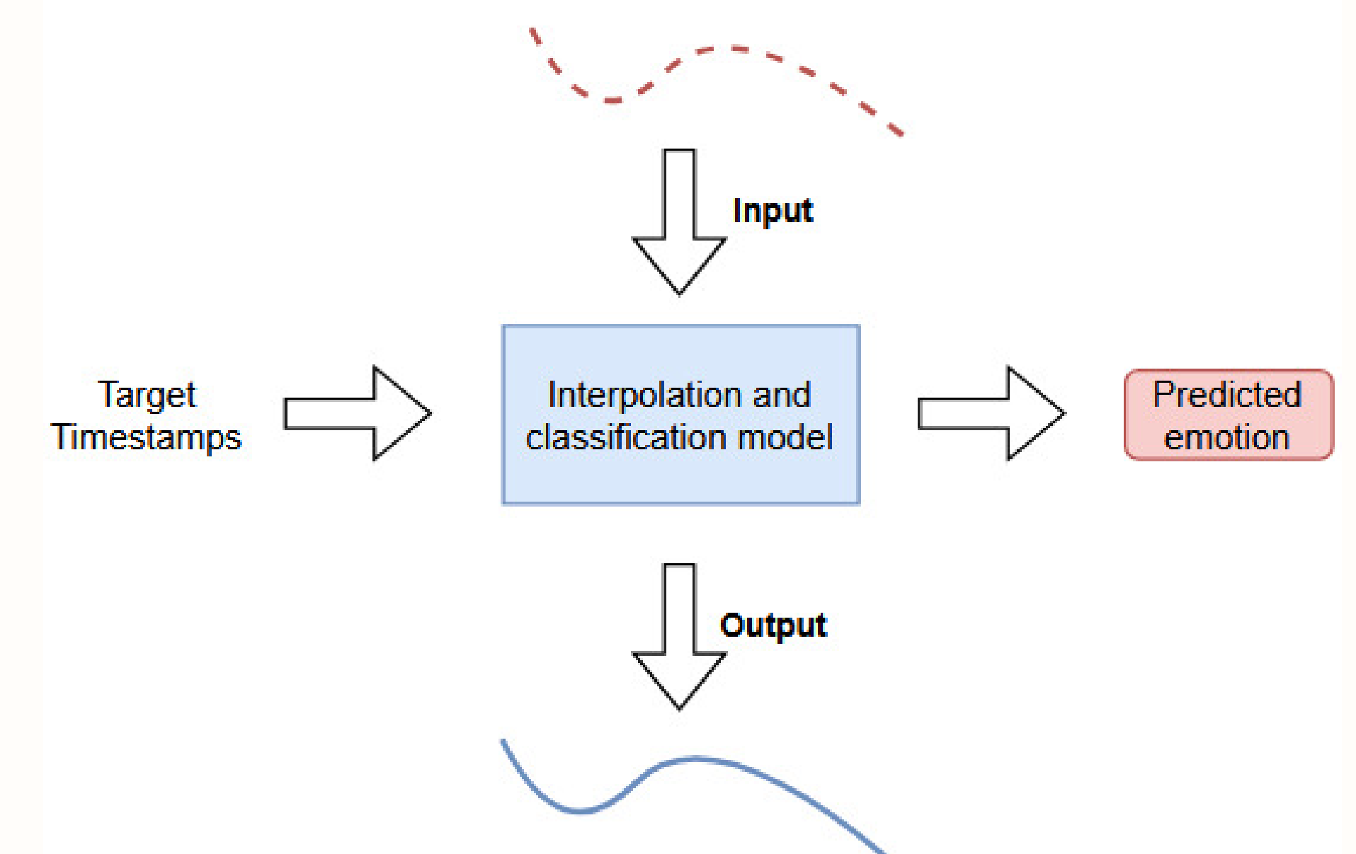
Figure 2: Workflow of the NCDE-based interpolation and classification pipeline: the sparse input sequence is converted to a continuous Hermite-spline control signal, integrated to obtain hidden states, then decoded for value reconstruction and classified for emotion probabilities.
