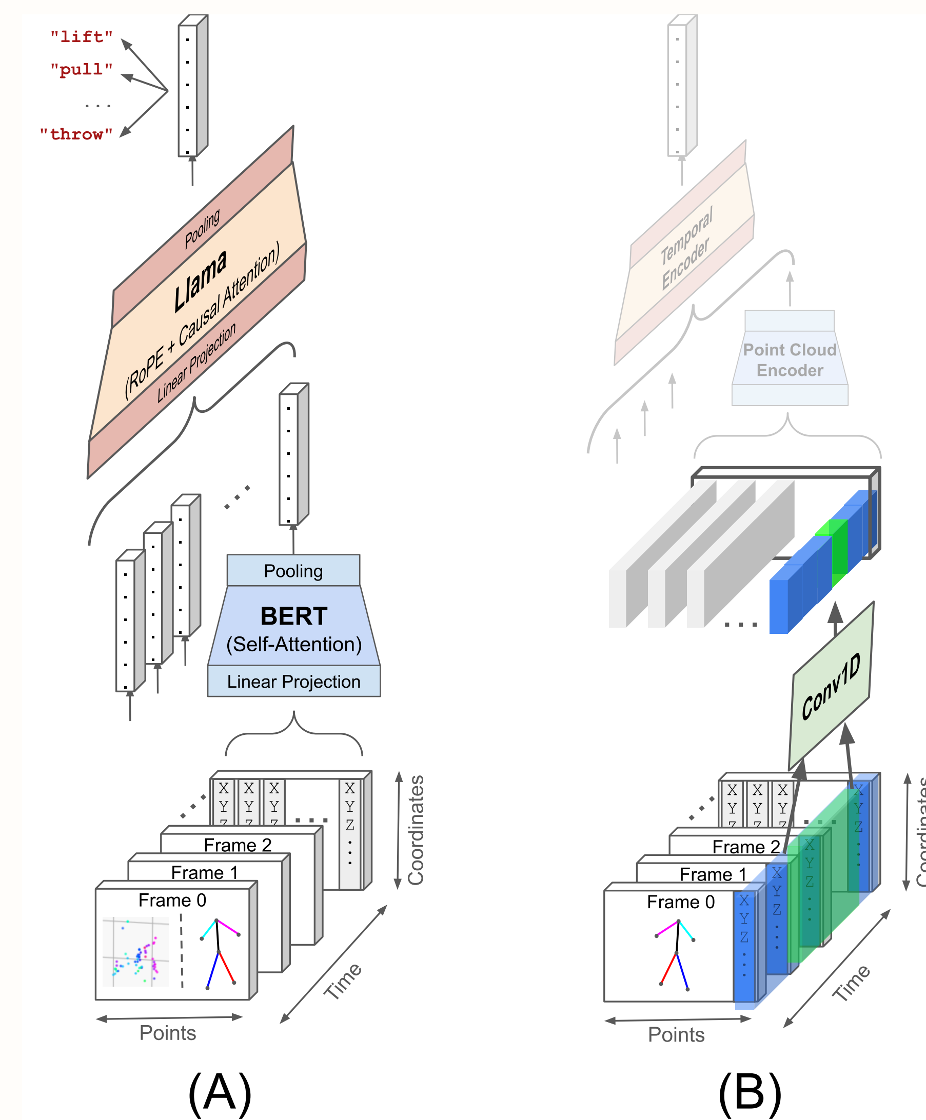
Figure 1: Dual Transformer pipeline
