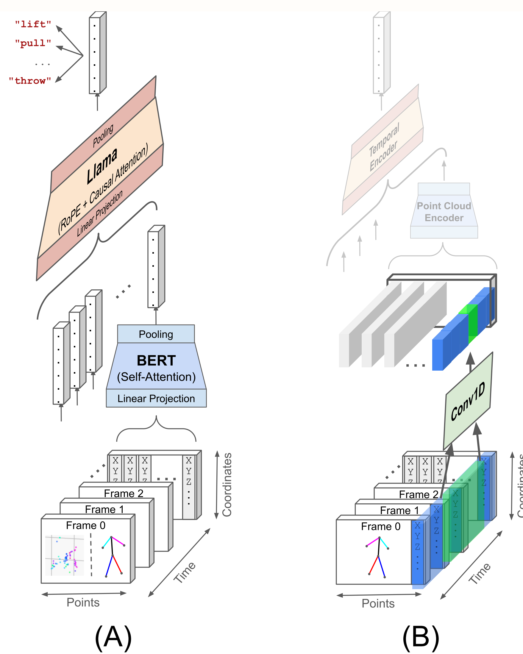
Figure 1: Dual Transformer pipeline
