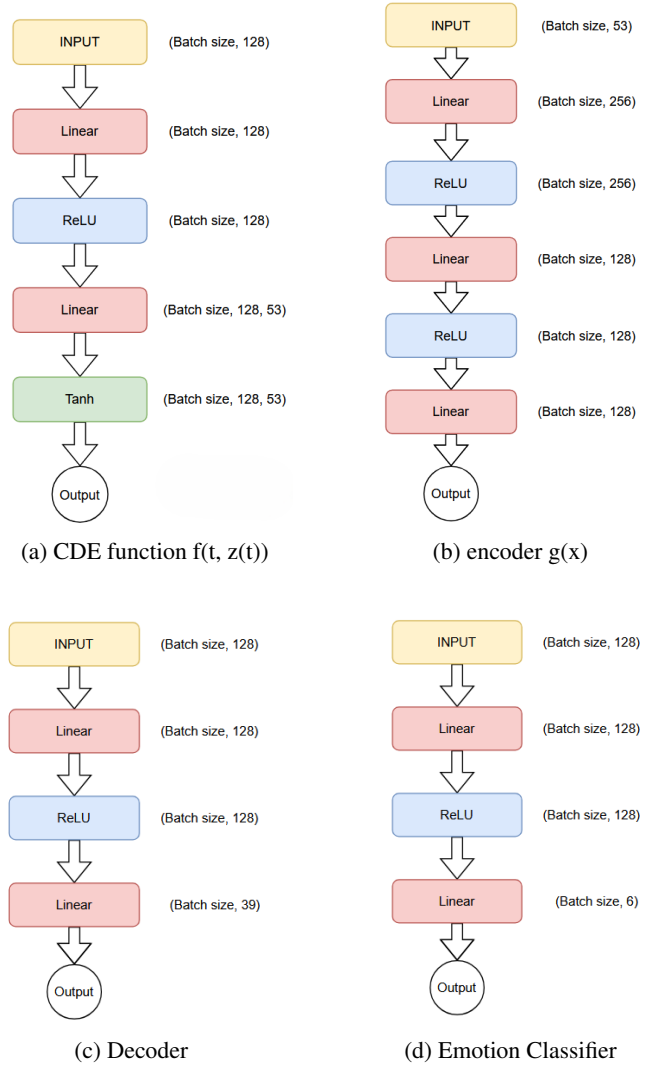
Figure 7: The four MLPs used in the model.
