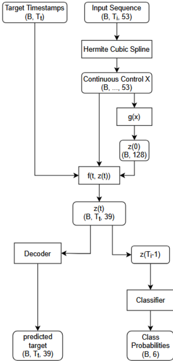
Figure 6: Workflow of the proposed method, it uses a differentiable hermite cubic spline which can be integrated to obtain the hidden state at arbitrary timestamps, the final hidden state is used to obtain class probabilities similar to RNNs.
