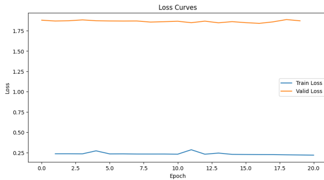
Figure 8: Training and validation loss plot.
