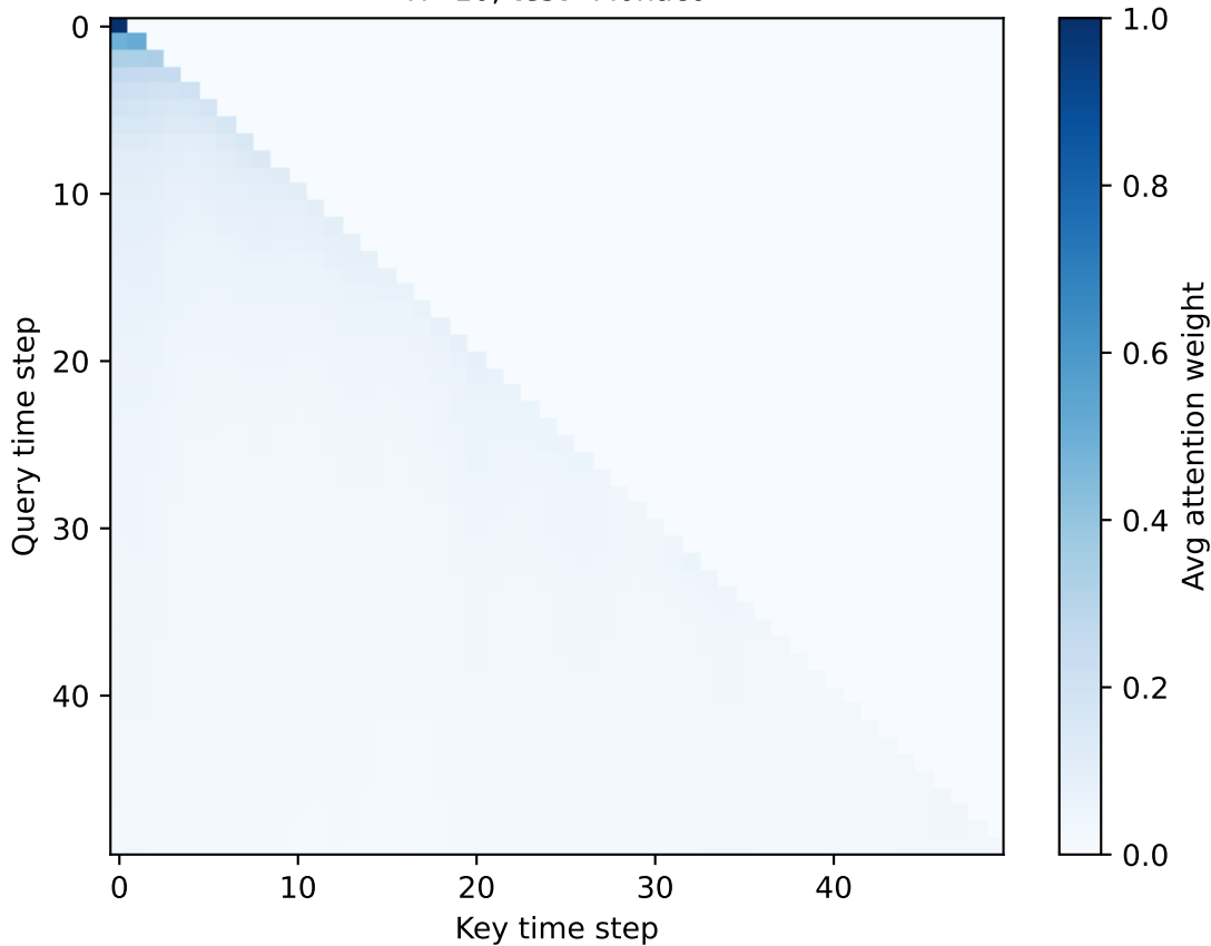
Transformer attention (mean over samples & layers) H=10, test=Monaco
