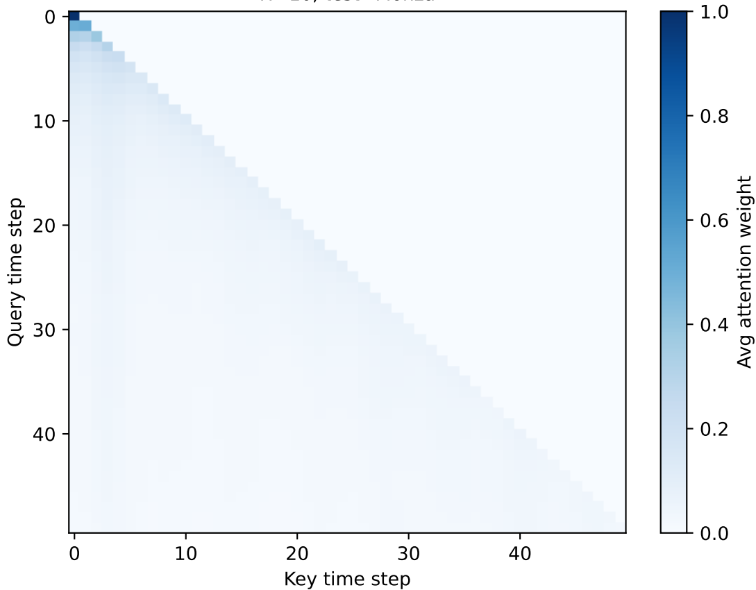
Transformer attention (mean over samples & layers) H=10, test=Monza
