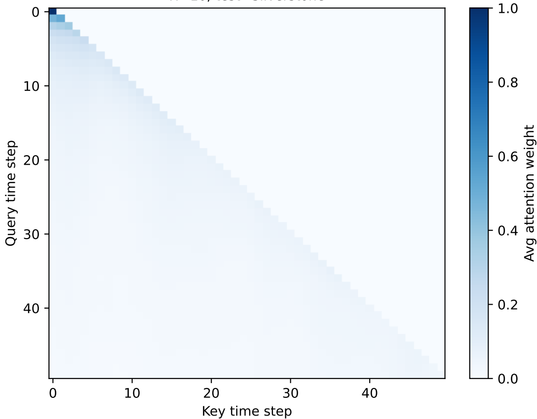
Transformer attention (mean over samples & layers) H=10, test=Silverstone
