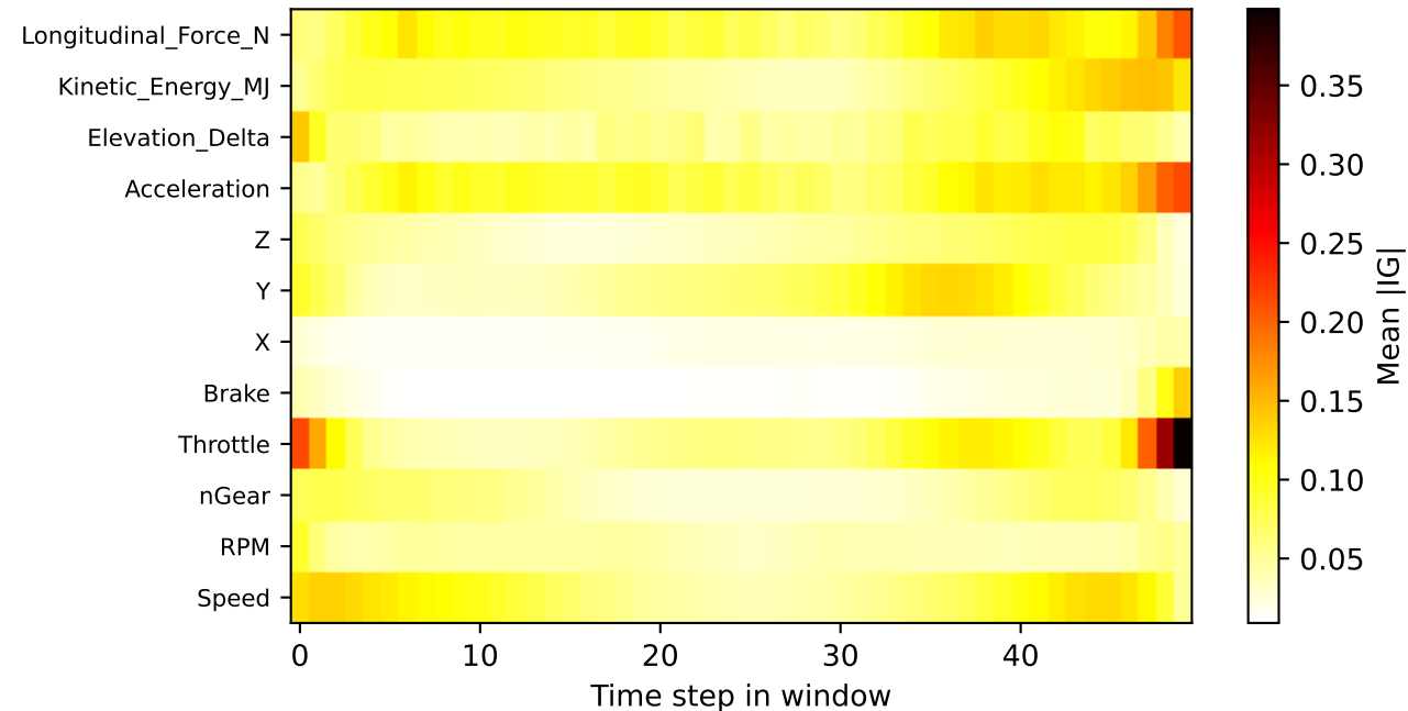
GRU — Integrated Gradients H=10, test=Monaco
