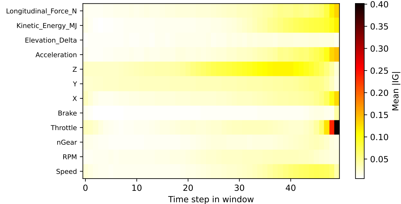
GRU — Integrated Gradients H=10, test=Silverstone
