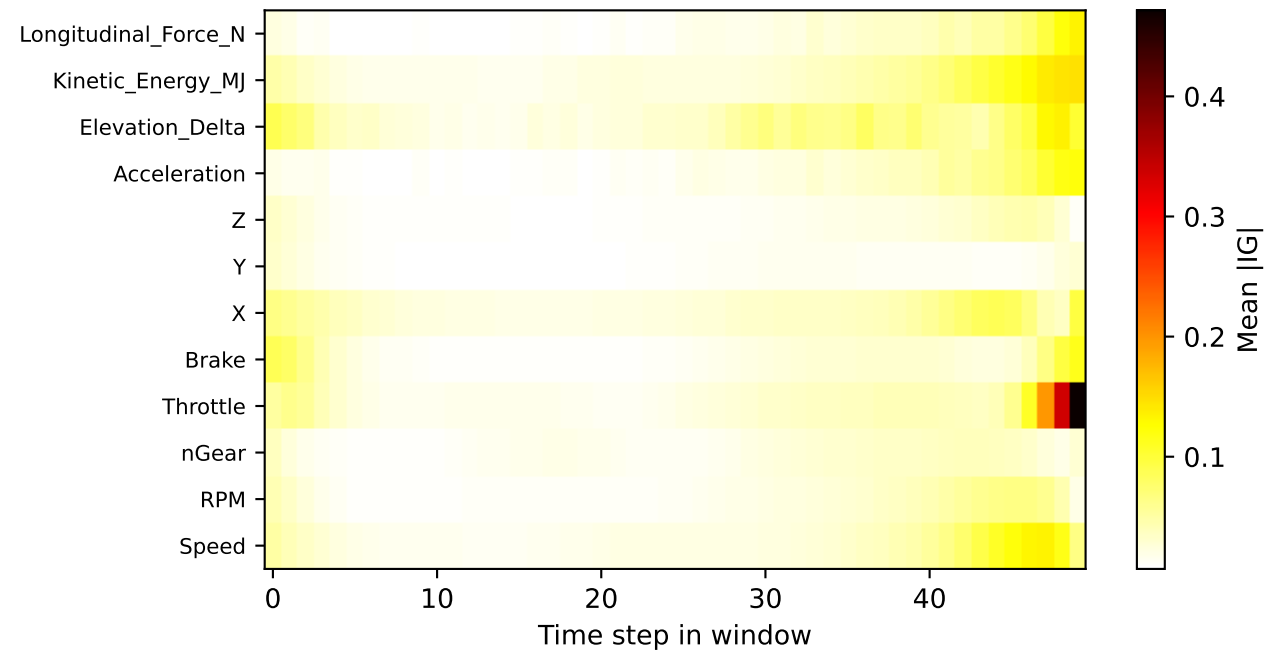
GRU — Integrated Gradients H=10, test=Suzuka
