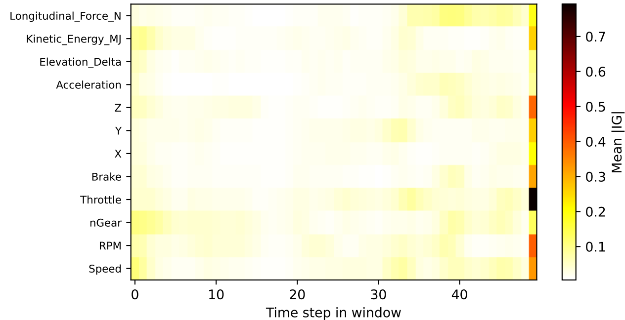
Transformer — Integrated Gradients H=10, test=Monaco
