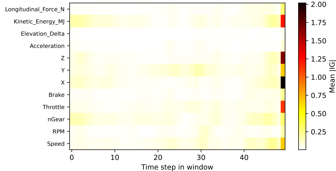
Transformer — Integrated Gradients H=10, test=Monza
