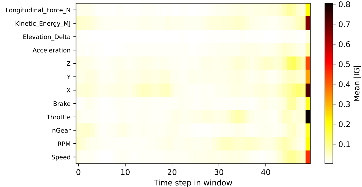
Transformer — Integrated Gradients H=10, test=Silverstone
