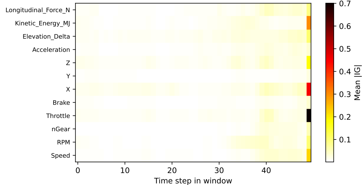
Transformer — Integrated Gradients H=10, test=Suzuka
