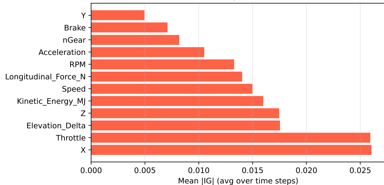
Feature importance (IG)
