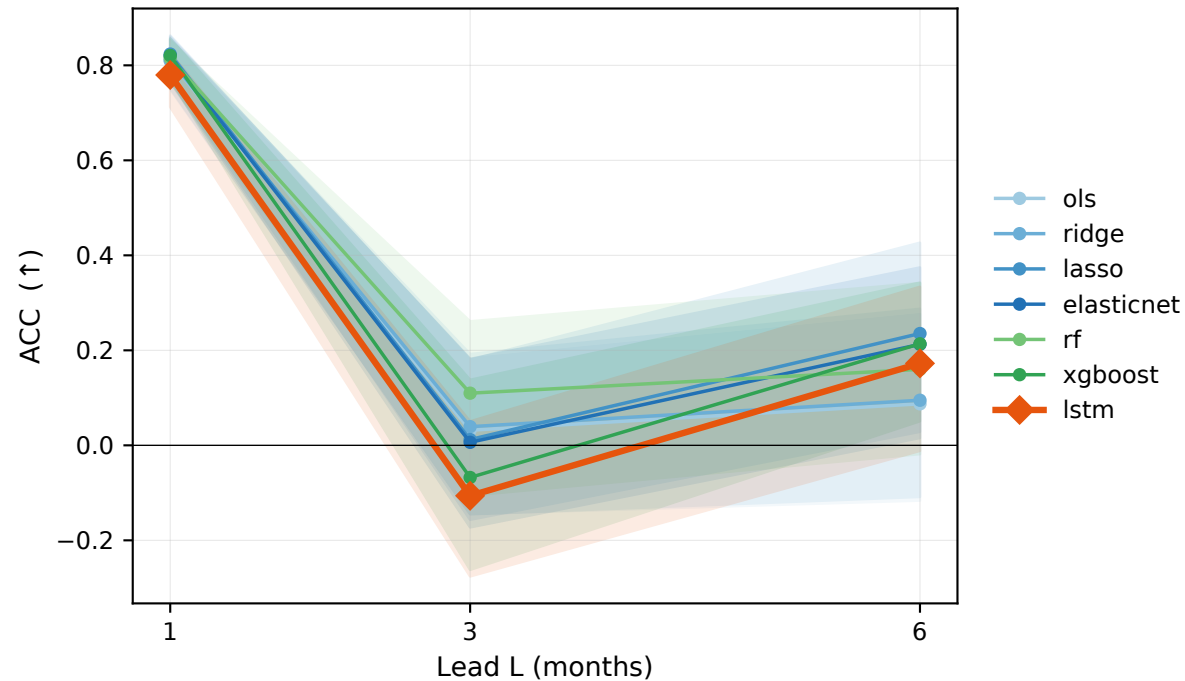
ACC vs lead · LSTM vs default
