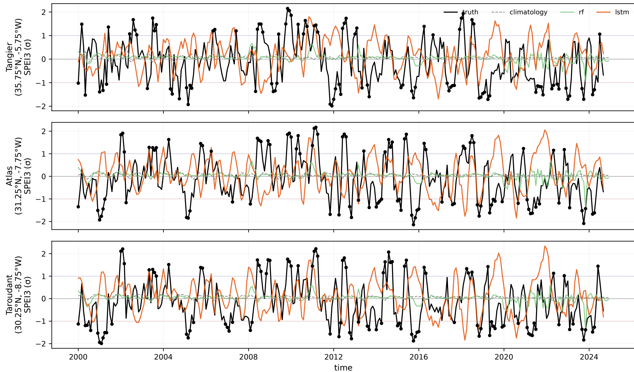
Time-series traces · OOS test window · L = 3 · LSTM vs default
