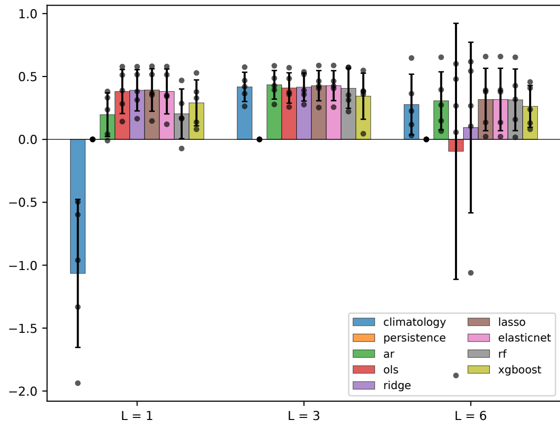
(b) MSSS vs persistence
