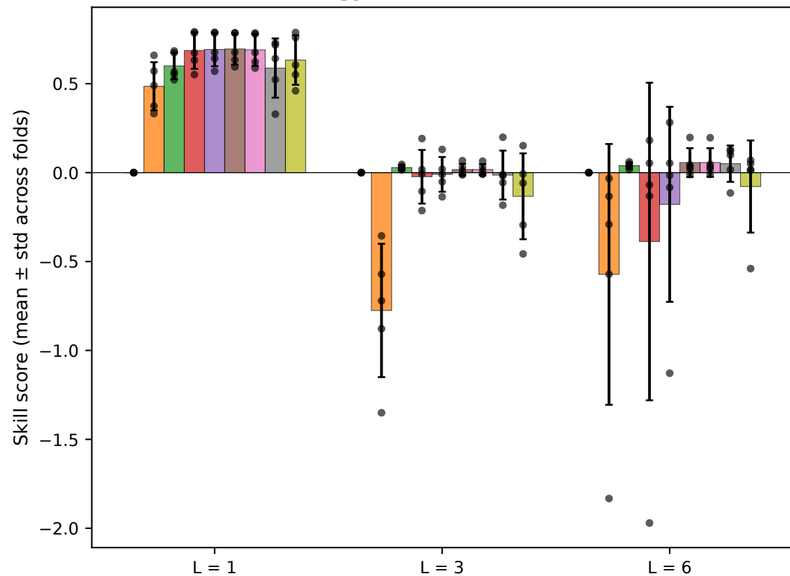
(a) MSSS vs climatology
