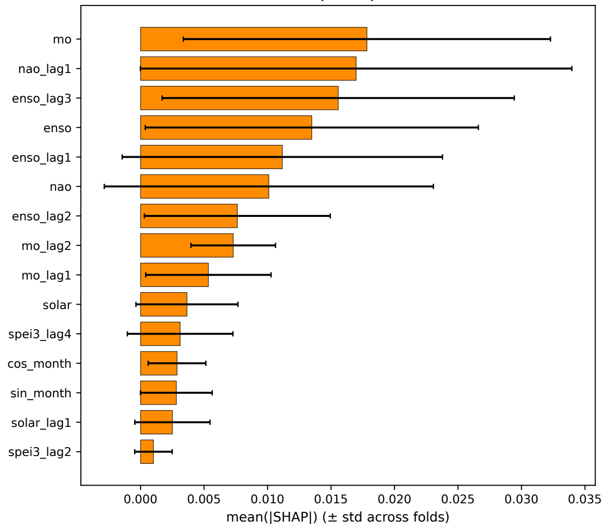
(b) XGBoost TreeSHAP mean(|SHAP|), L=3
