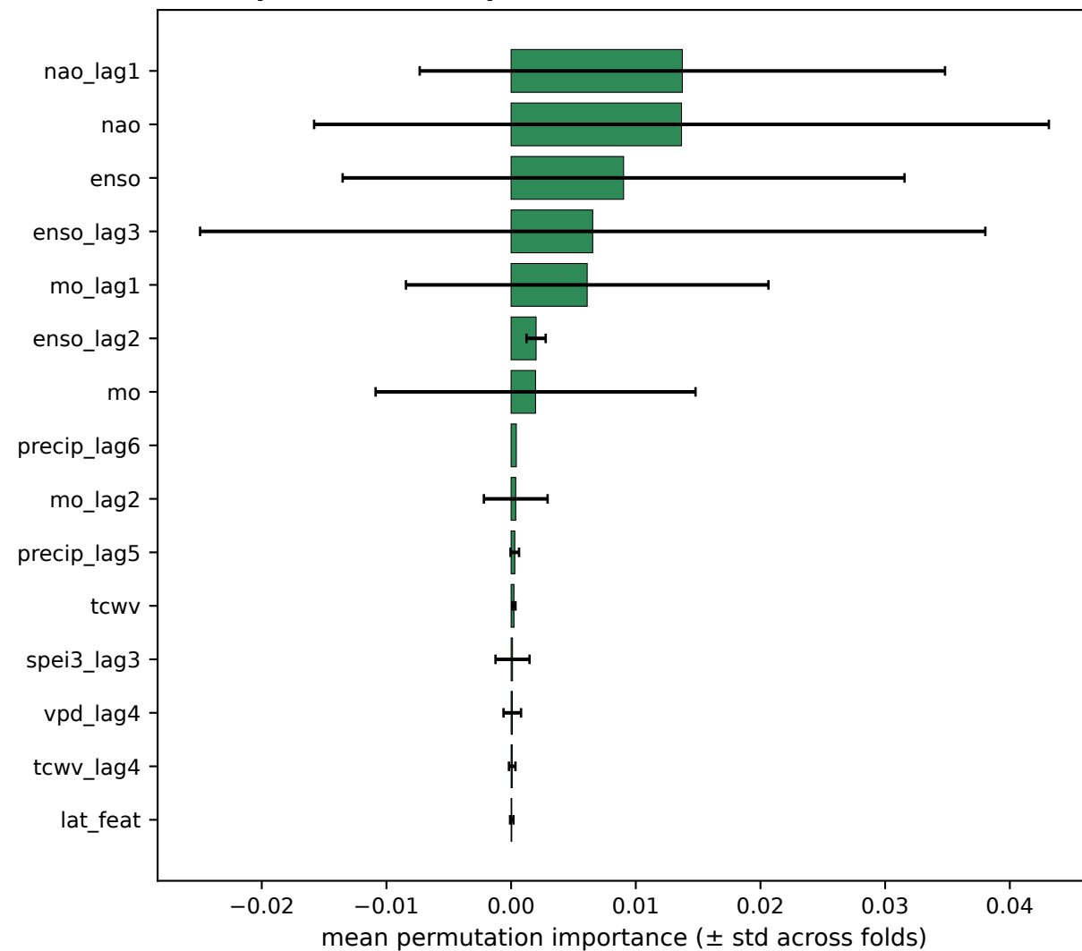
(a) RF permutation importance, L=3
