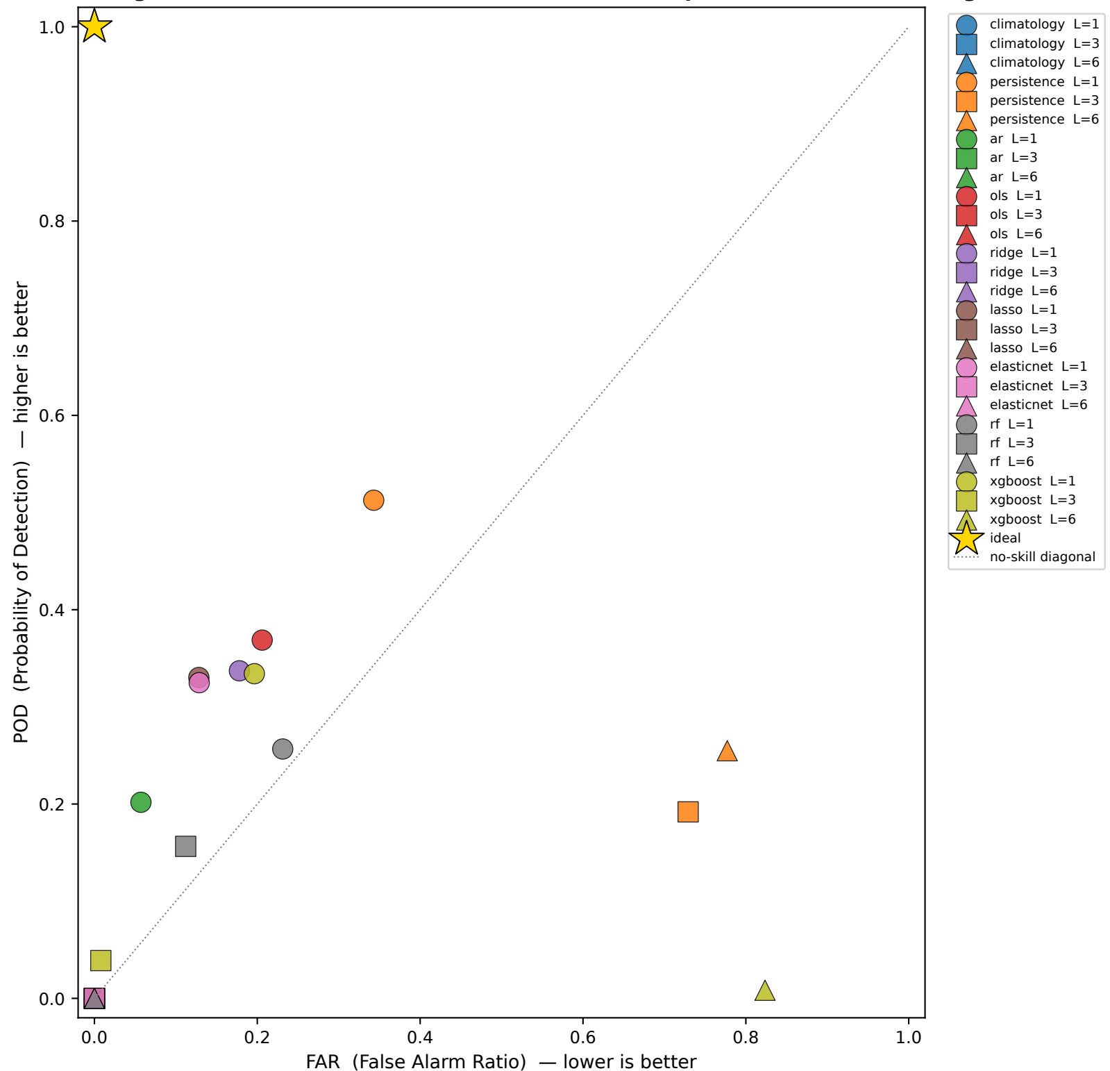
Drought detection (SPEI3 < -1.0) — POD vs FAR · experiment: winter-training
