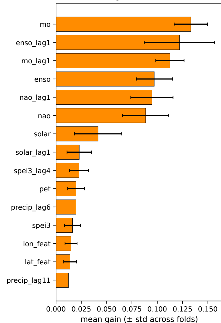
(c) XGBoost gain, L=3
