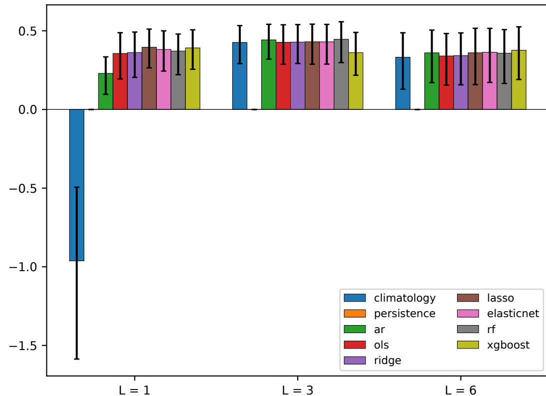
(b) MSSS vs persistence
