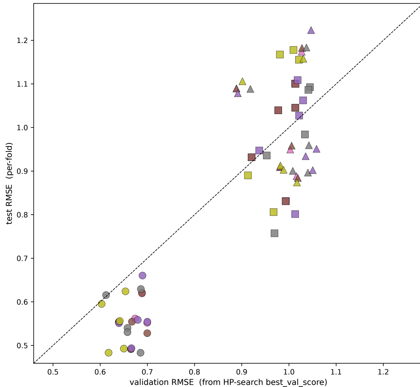
(a) Validation vs Test
