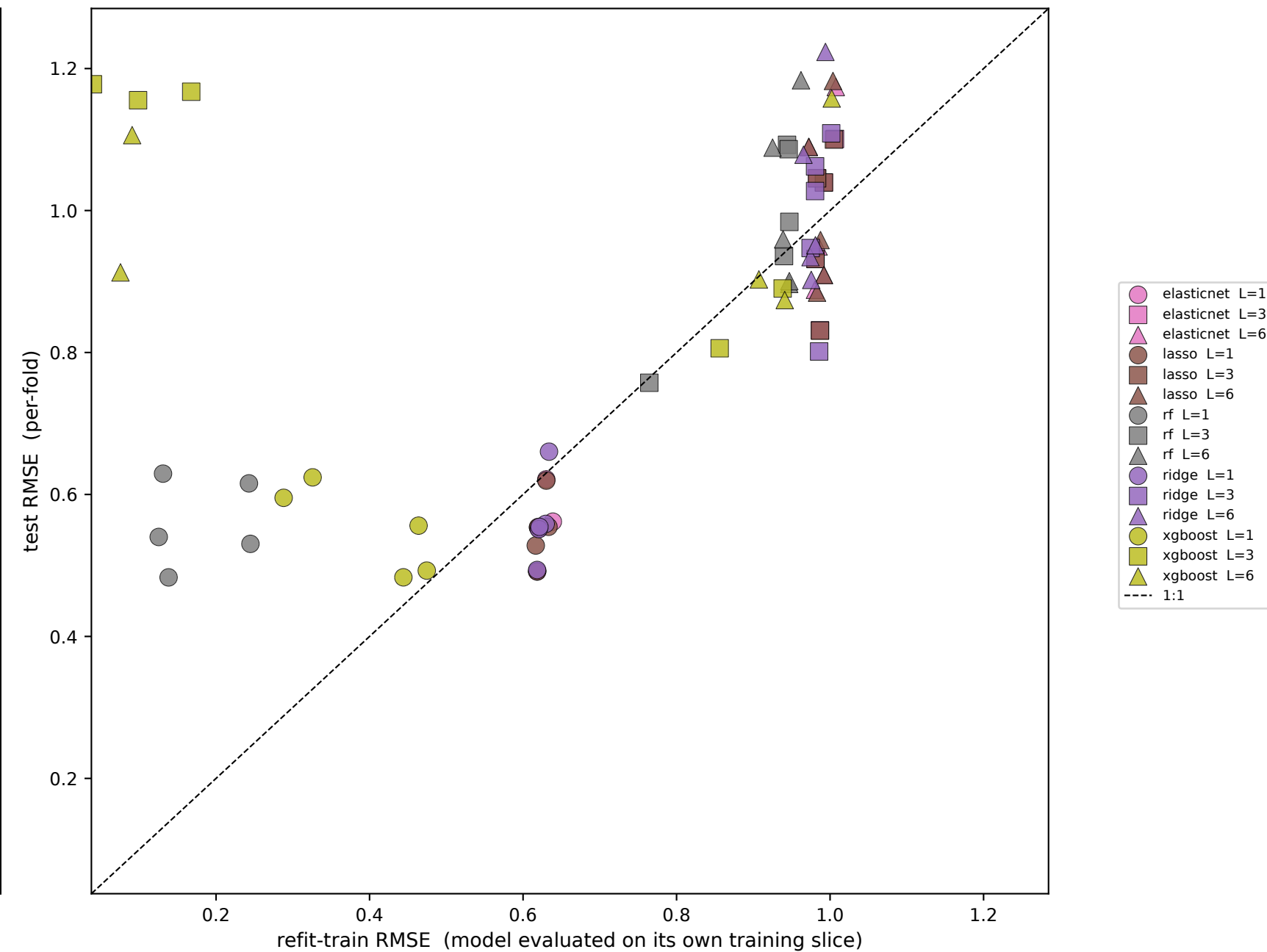
(b) Refit-Train vs Test
