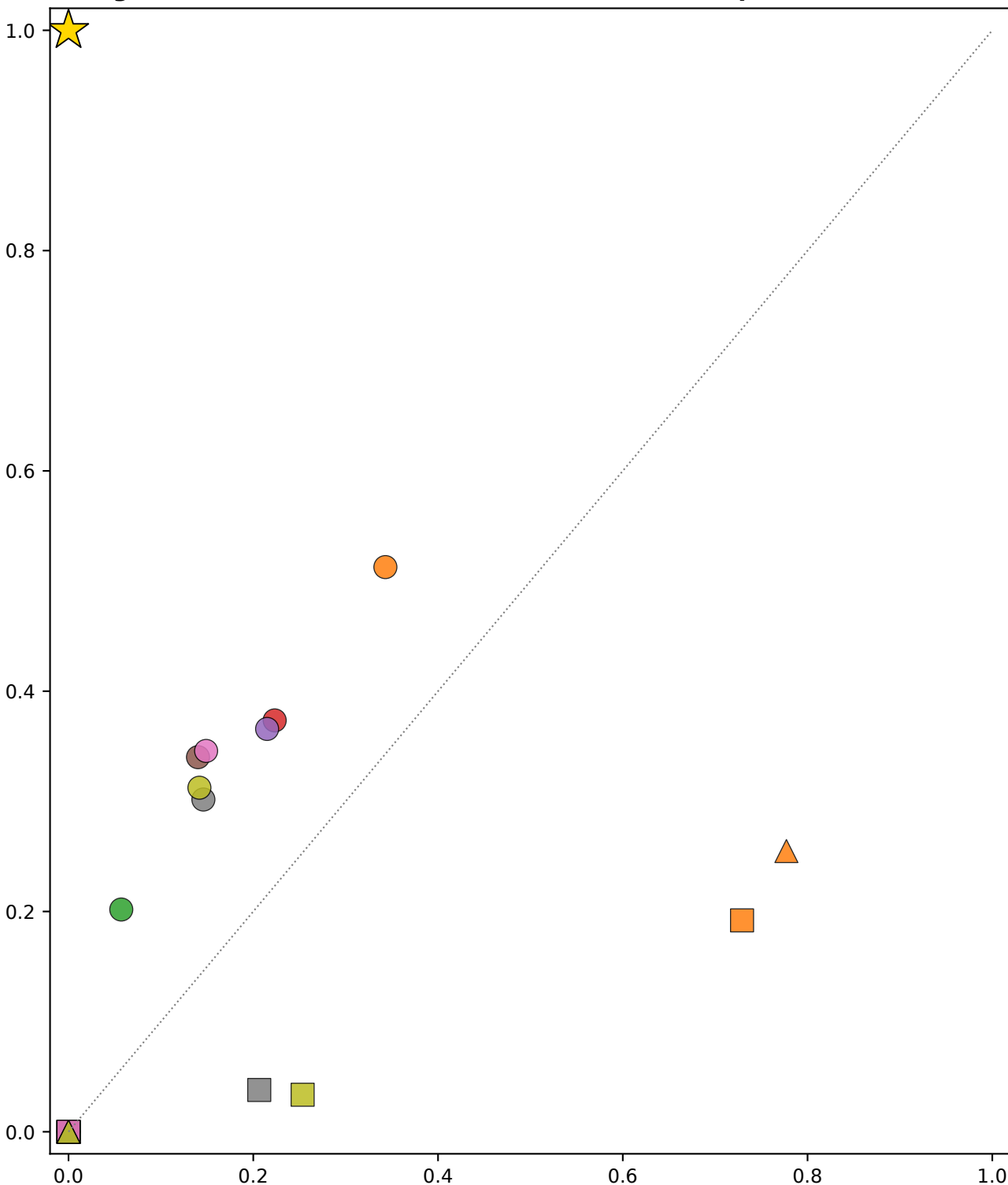
Drought detection (SPEI3 < -1.0) — POD vs FAR · experiment: default
