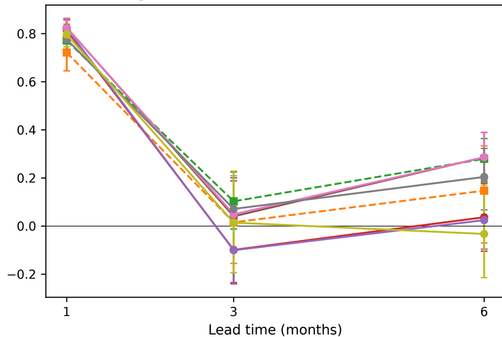
(a) Anomaly correlation
