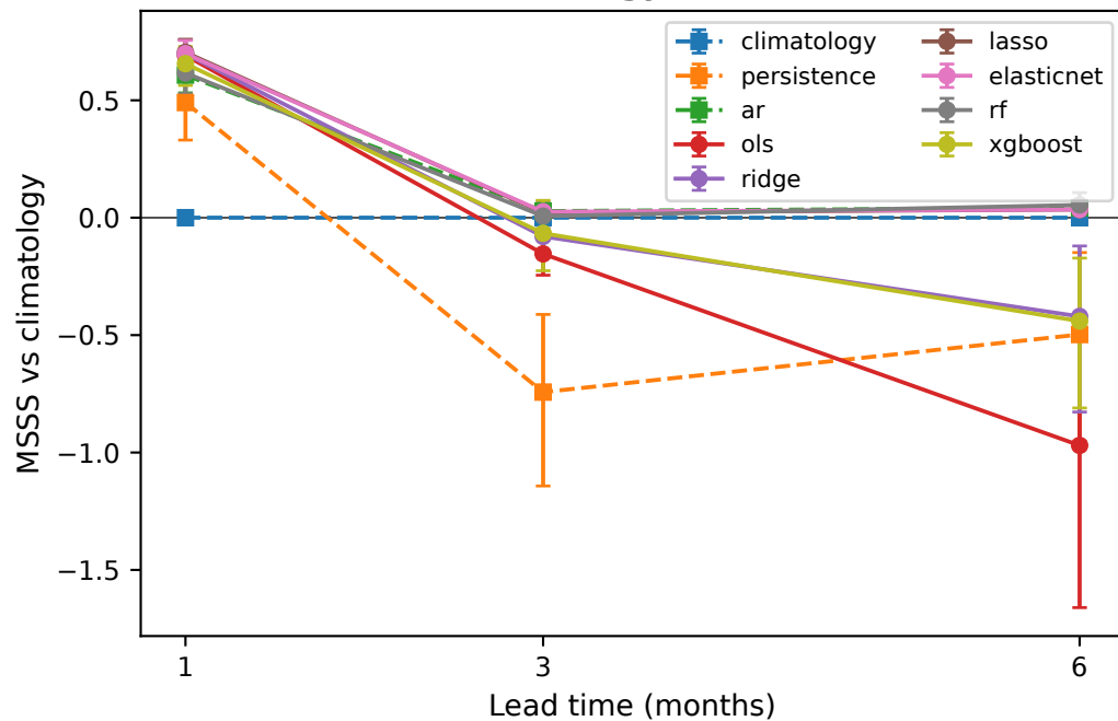
(b) Skill score vs climatology
