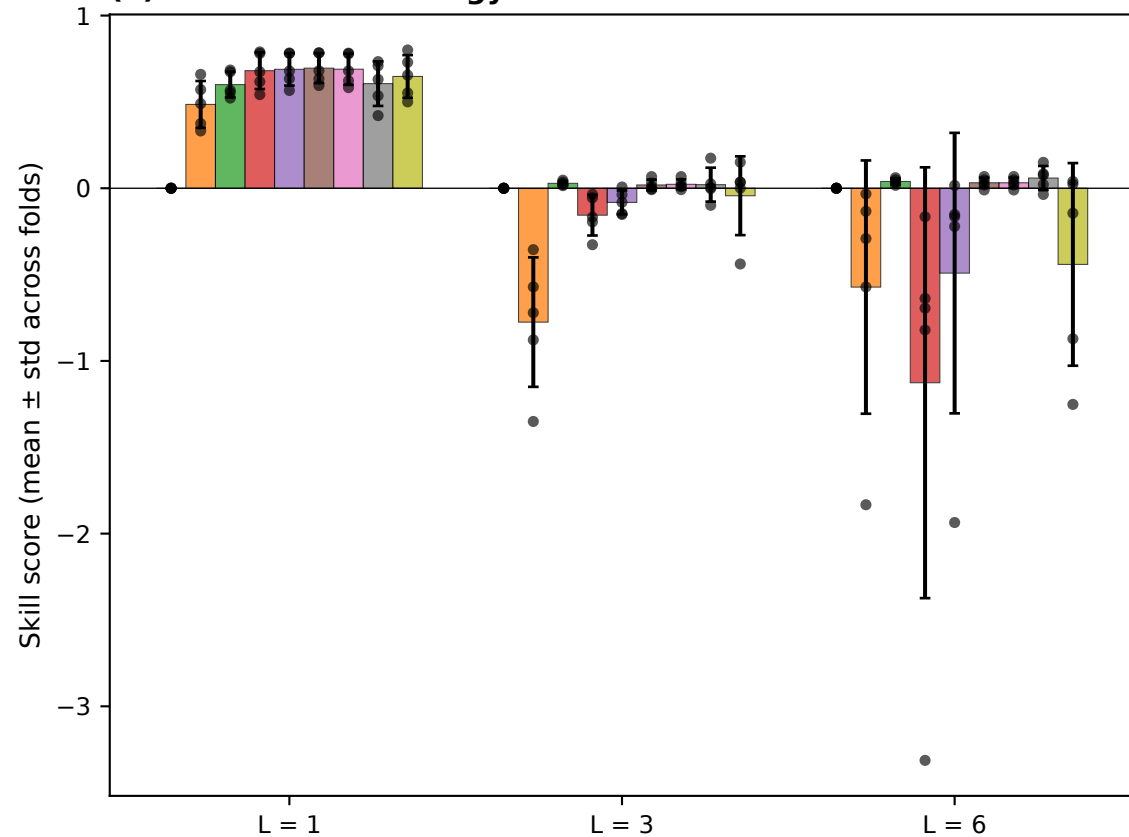
(a) MSSS vs climatology
