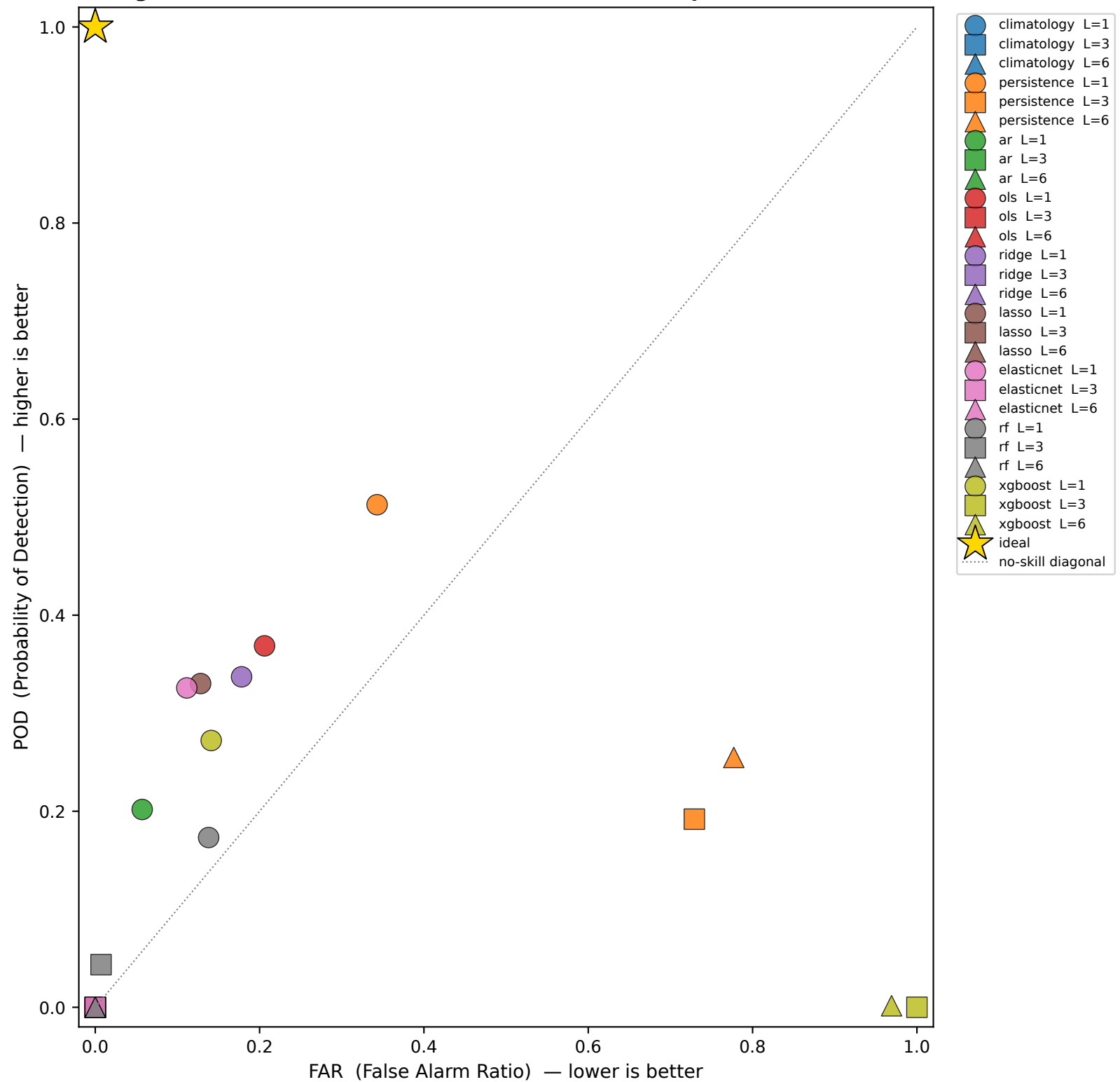
Drought detection (SPEI3 < -1.0) — POD vs FAR · experiment: winter-HPenhanced
