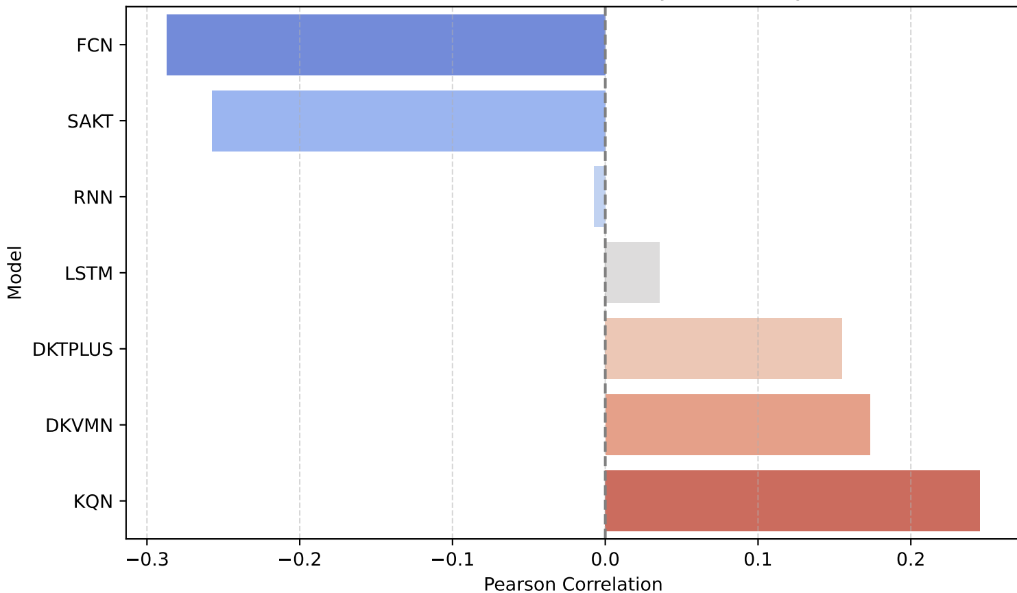
Correlation between Dataset Density and AUC by Model
