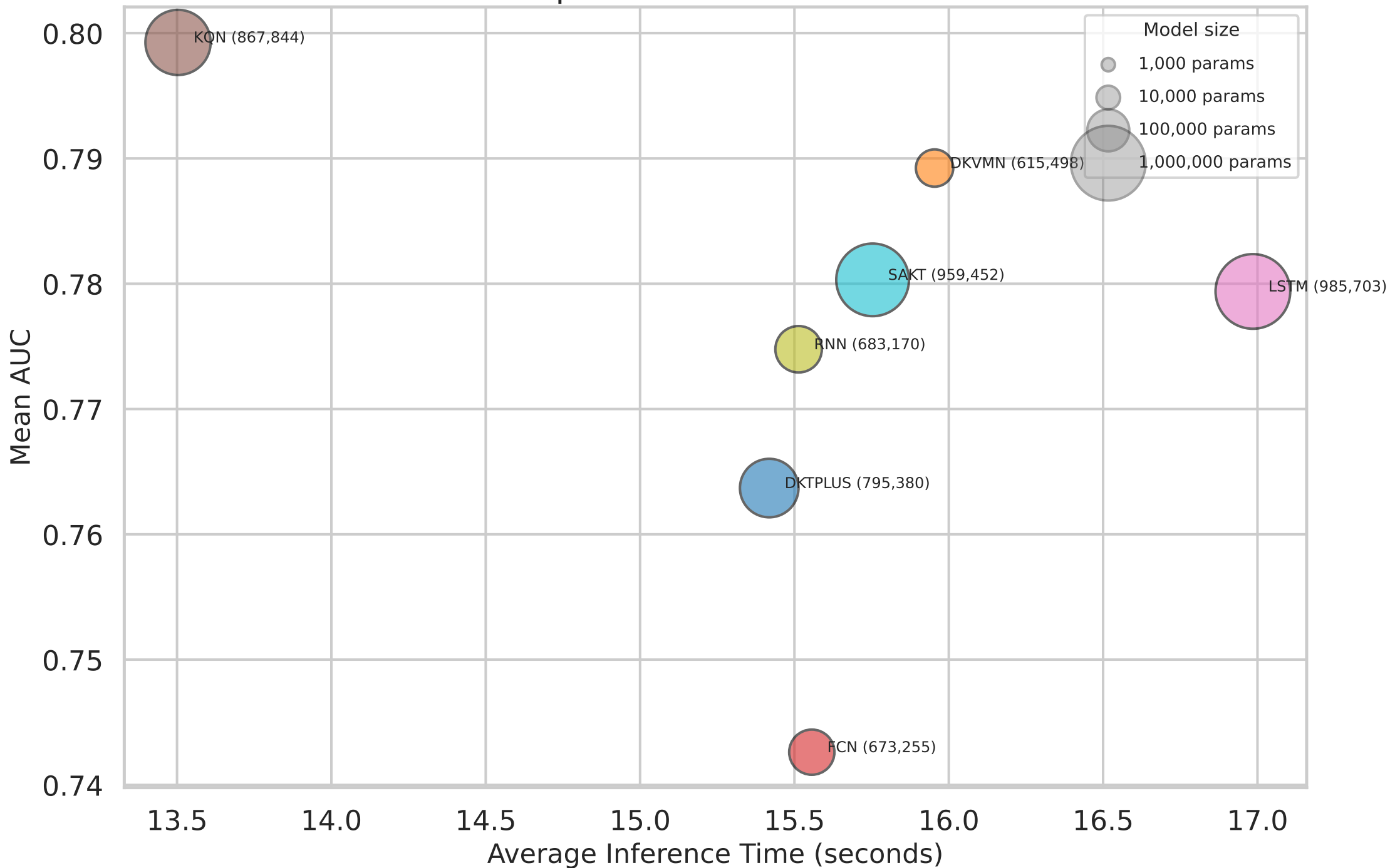
Models Comparison- Inference Time vs AUC
