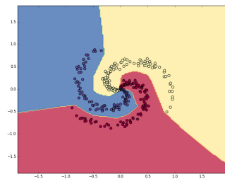
Neural network
