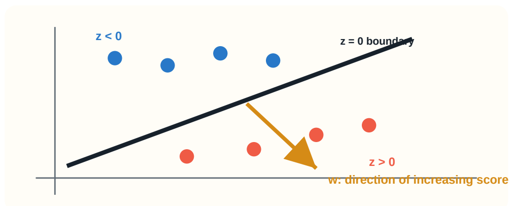
Figure 5: A neuron first creates a linear boundary and then converts signed distance-like scores into responses. Course schematic; the biological-neuron analogy commonly used in neural-network introductions is also illustrated by Stanford CS231n (Li et al., n.d.).
