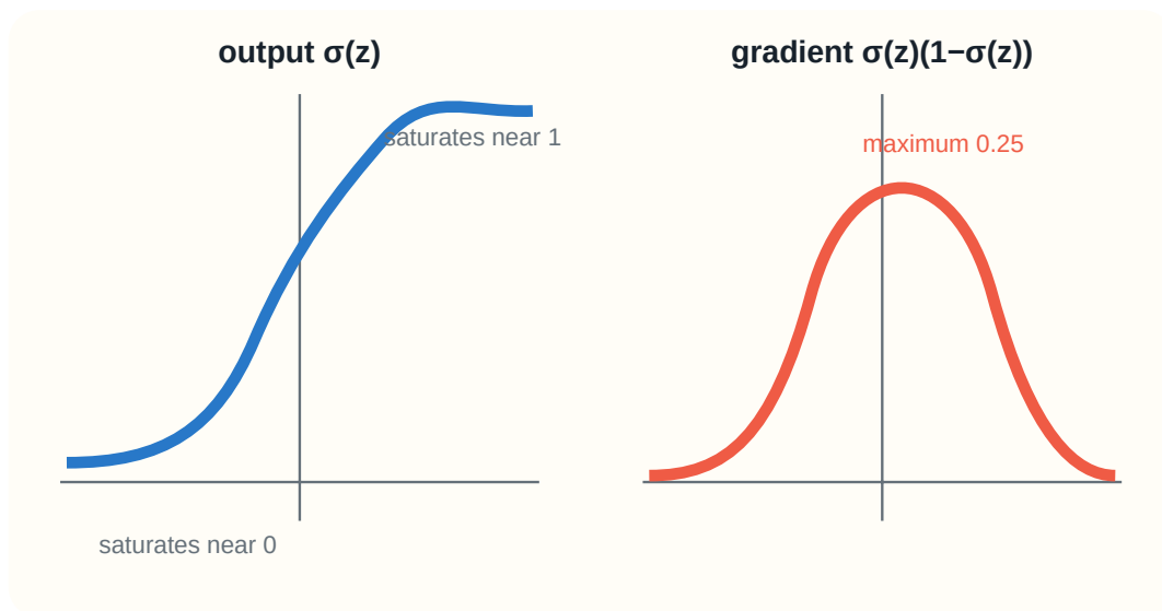
Figure 7: Sigmoid output and derivative. The derivative is at most 1/4 and approaches zero for inputs far from the origin.
