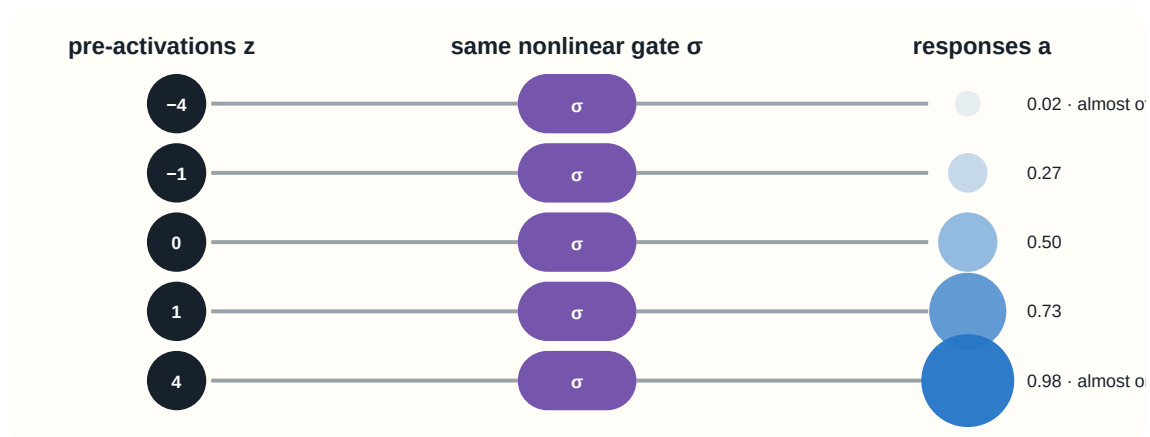
Figure 6: Several neurons apply the same activation to different pre-activations. Some units respond strongly and others are suppressed, creating a new feature vector rather than another linear copy of the input.
