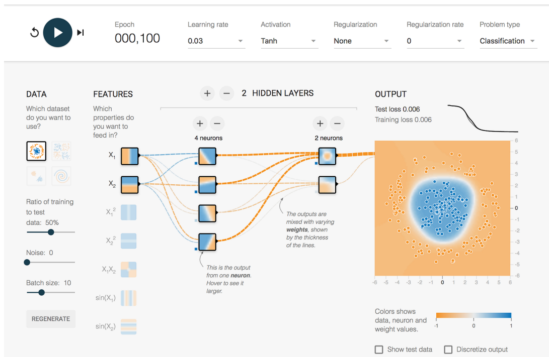
Figure 3: TensorFlow Playground fitting concentric classes with a neural network. The visualization exposes the learned output of each hidden unit.
