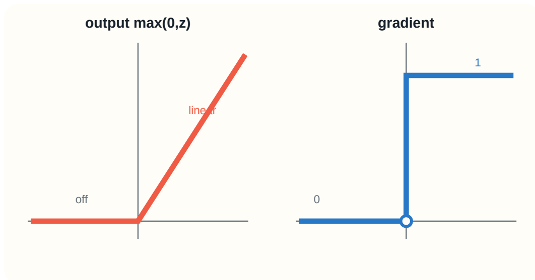
Figure 9: ReLU output and derivative. Positive values pass unchanged, while negative values and their local gradients are suppressed.
