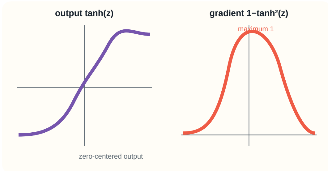
Figure 8: Tanh output and derivative. Tanh is zero-centered but still saturates at both extremes.
