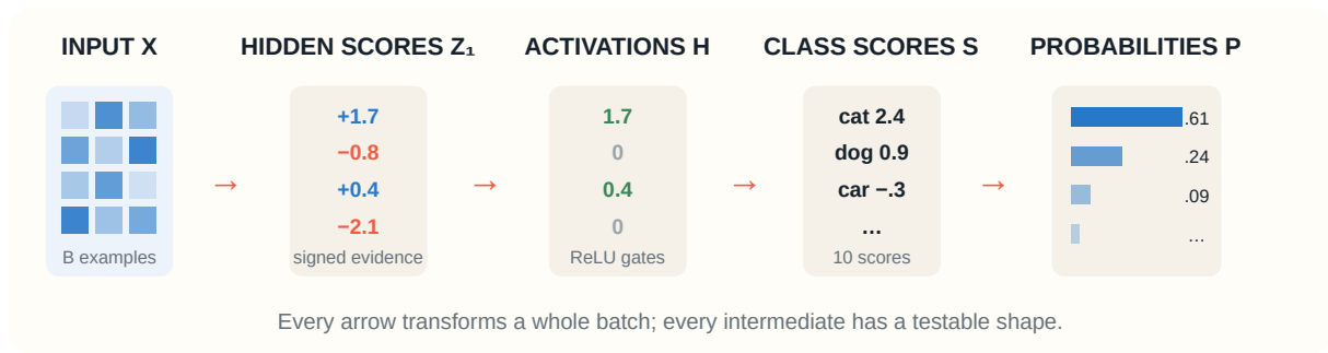
Figure 11: The two-layer forward pass shown as explicit computational stages, from a batch of inputs to class scores.
