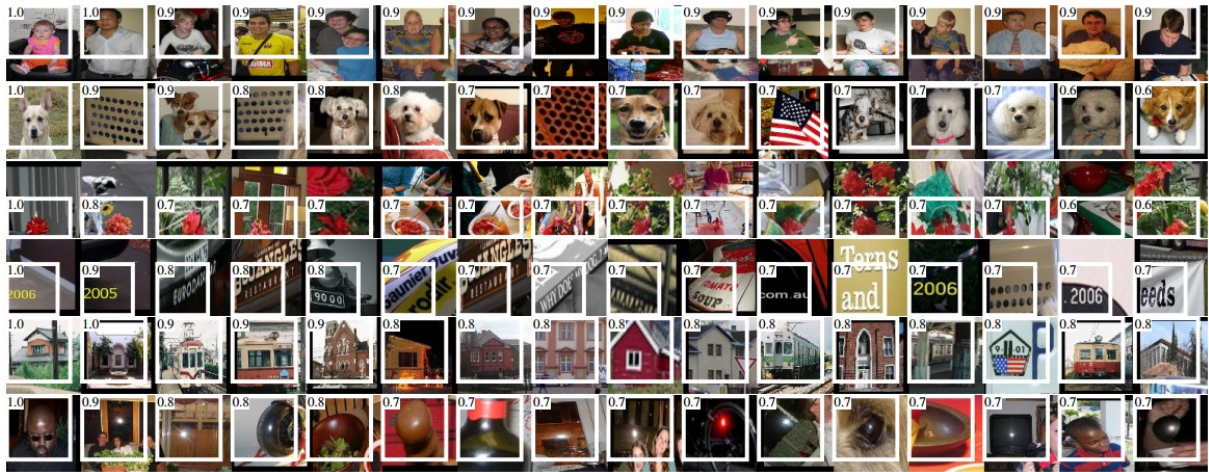
Figure 13: Image patches that maximally activate selected AlexNet pool5 units. The white values report activation magnitudes, making clear that a representation contains graded numerical responses rather than only on/off symbols. Source: Stanford CS231n (Li et al., n.d.).
