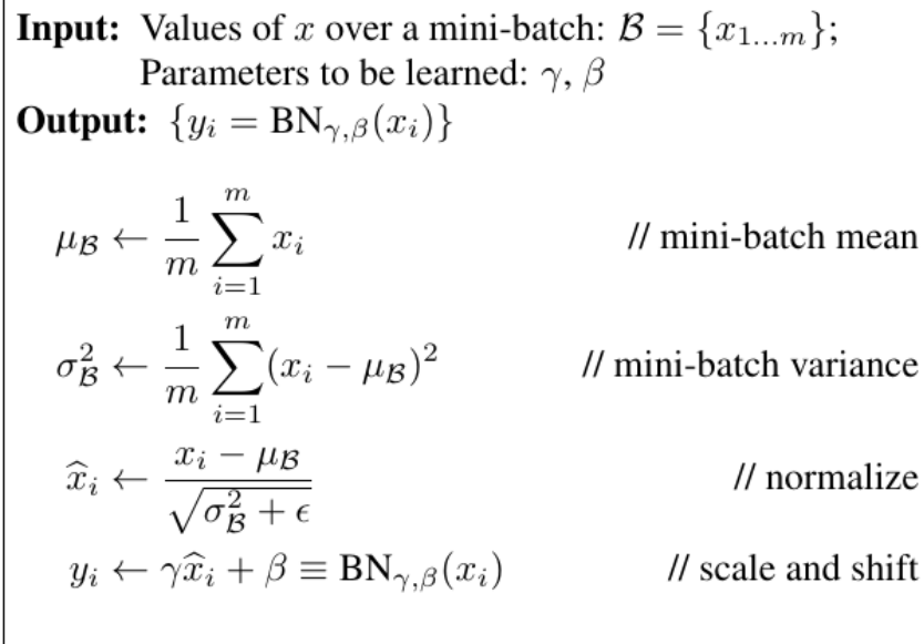
Figure 4: Algorithm 1 from the original BatchNorm paper gives the complete minibatch transformation. Source: Ioffe and Szegedy (2015).
