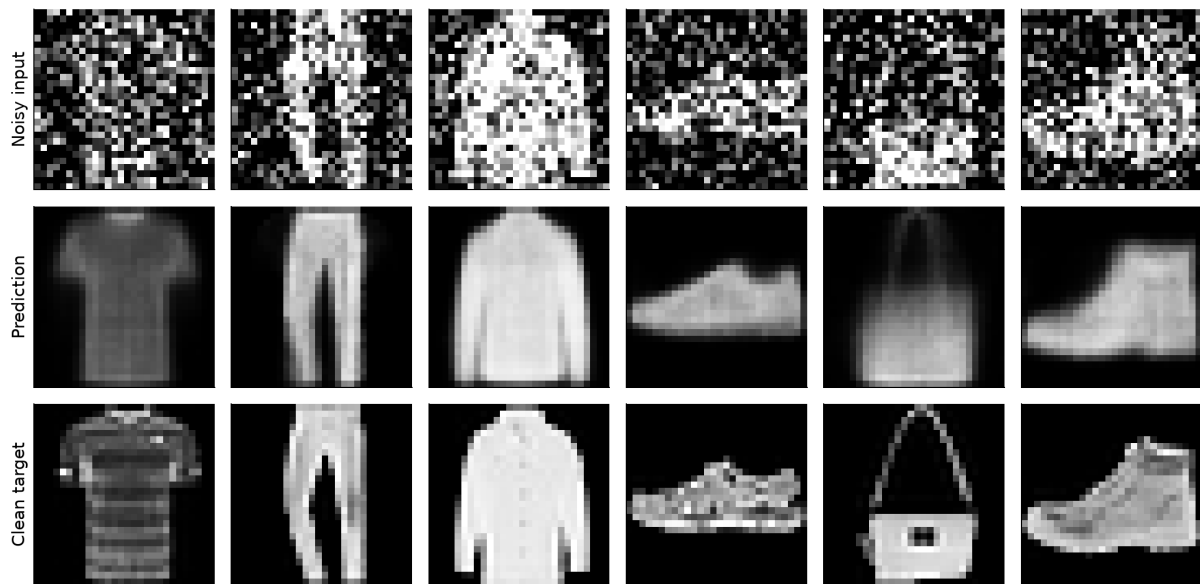
Figure 11: The exact six noisy inputs, model predictions, and clean targets shown in the lecture, aligned for comparison.
