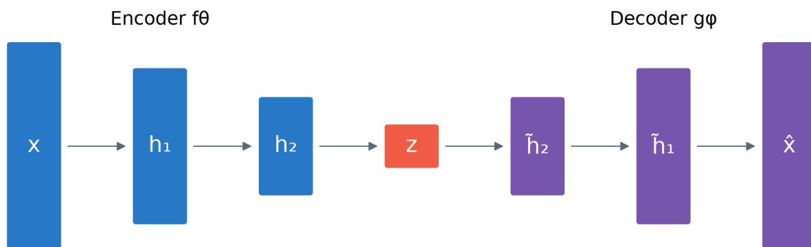
Figure 4: The lecture’s hourglass reconstructed for reading: each rounded vertical bar is a complete state, and height indicates relative coordinate count. Arrows denote deterministic transformations. Course diagram.
