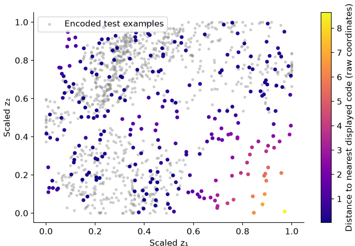
Figure 14: The lecture’s 250 uniform probes over a rectangle spanning the central coordinate ranges. Gray points are encoded test examples; color measures raw-coordinate distance to the nearest of those 1,000 examples.
