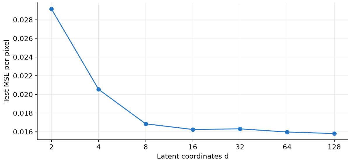
Figure 7: Measured test MSE averaged across pixels and images. The early gains are large, followed by a broad plateau.
