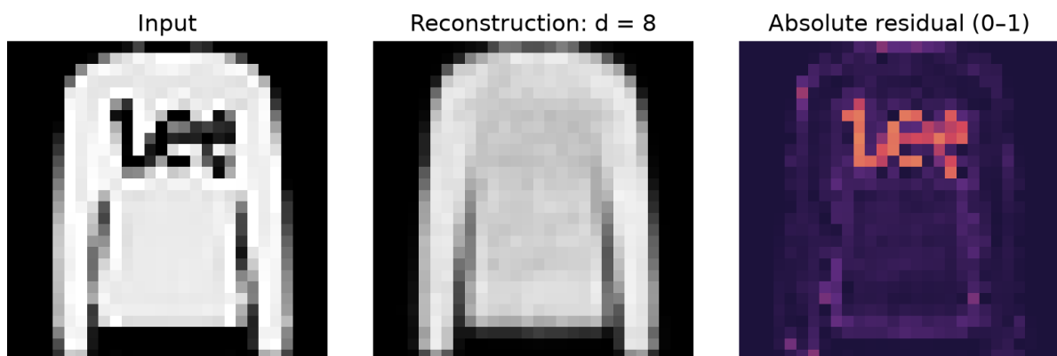
Figure 6: The pullover input, its eight-dimensional reconstruction, and the absolute-error map used in the lecture explorer. Dark purple means little error; warm yellow means large absolute pixel discrepancy on a fixed 0–1 scale.
