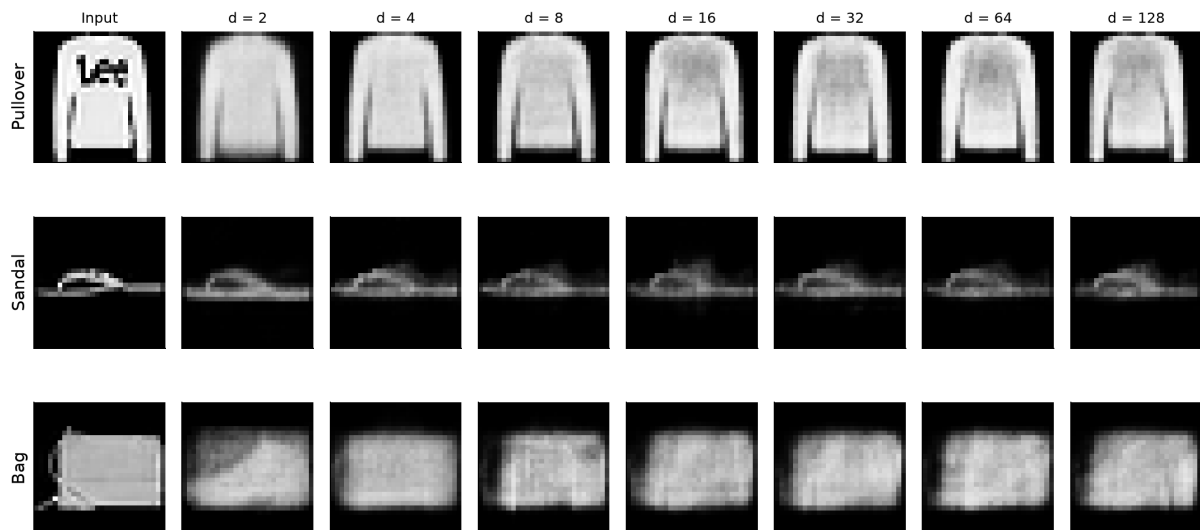
Figure 5: The same three held-out inputs across every latent width. The pullover reproduces the lecture’s filmstrip; sandal and bag expose different reconstruction difficulties. Course-trained outputs, not drawn predictions.
