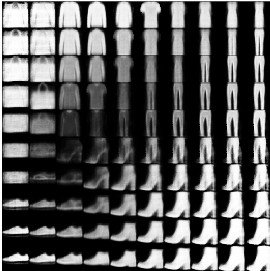
Figure 15: The lecture’s 10×10 decoder atlas. Left to right increases the first latent coordinate; top to bottom decreases the second. All cells are outputs from the same trained two-dimensional decoder.
