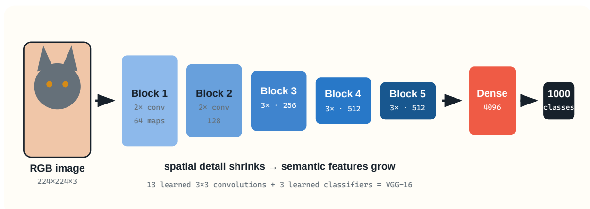
Figure 6: A course schematic of VGG-16. The architecture contains 13 convolutional layers followed by three learned classifiers and was trained for large-scale ImageNet recognition (Simonyan and Zisserman 2015). We will derive convolution, pooling, and every block later in the course.
