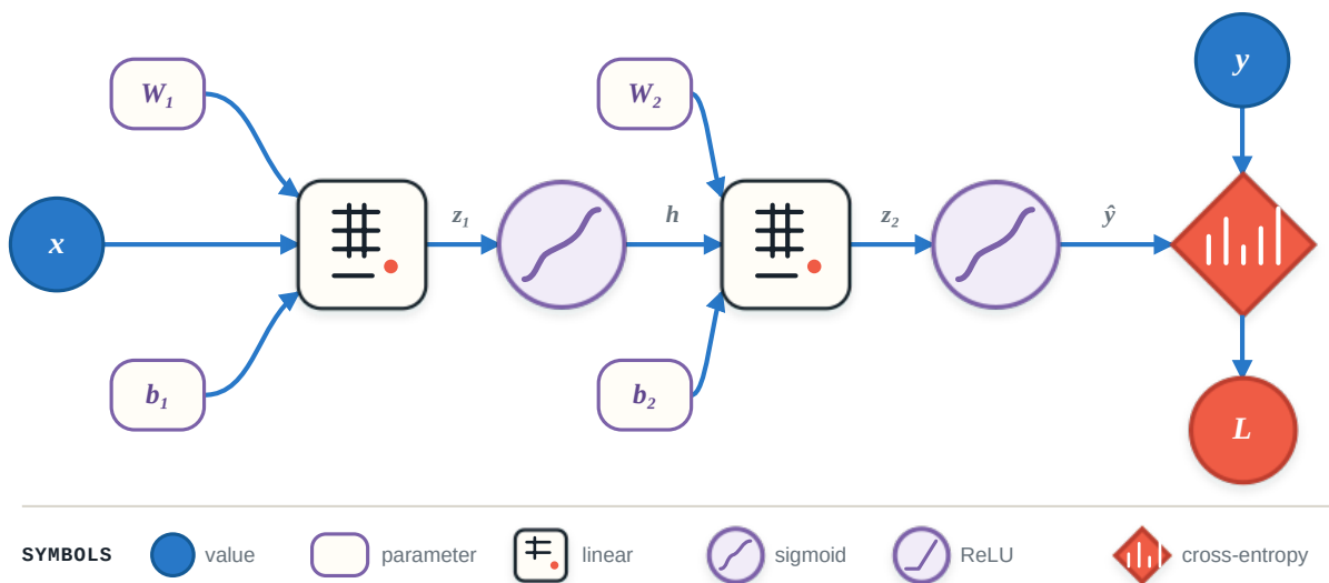
Figure 2: The symbolic graph used throughout the lecture. Values are blue circles, parameters are purple rounded rectangles, affine maps are square blocks, activations are purple circles, and the loss is coral.
