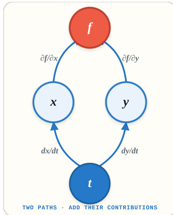
Figure 8: Two paths connect t to f . Each path contributes one product of local derivatives.
