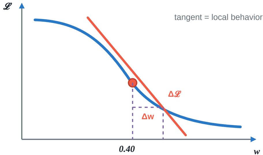
Figure 3: A local perturbation is compared with the tangent prediction at one point.
