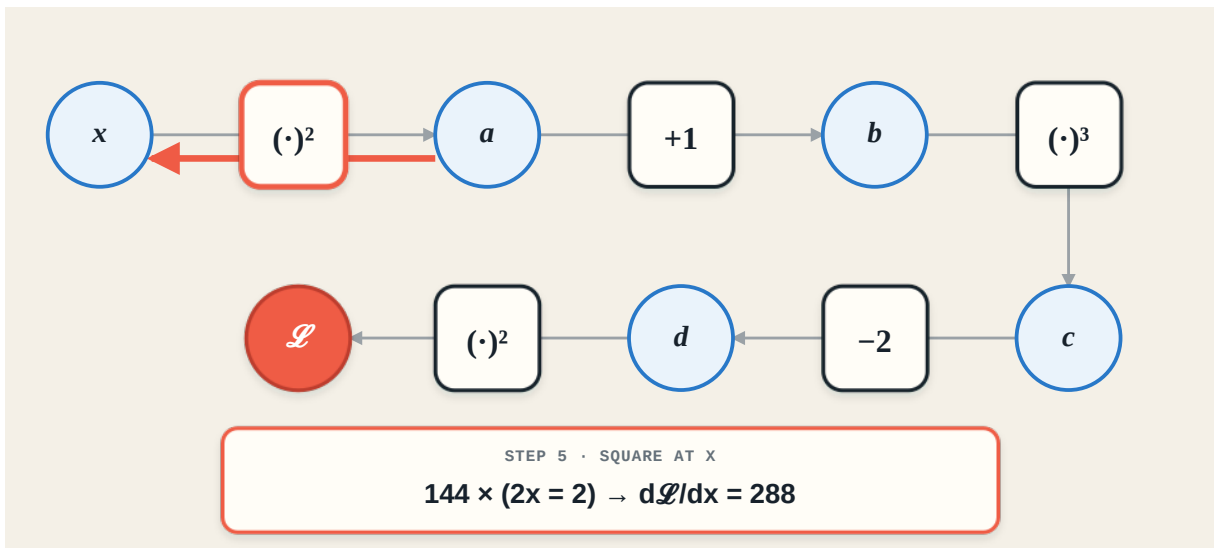
Figure 6: The final backward state highlights the local computation that sends the derivative 288 to x .
