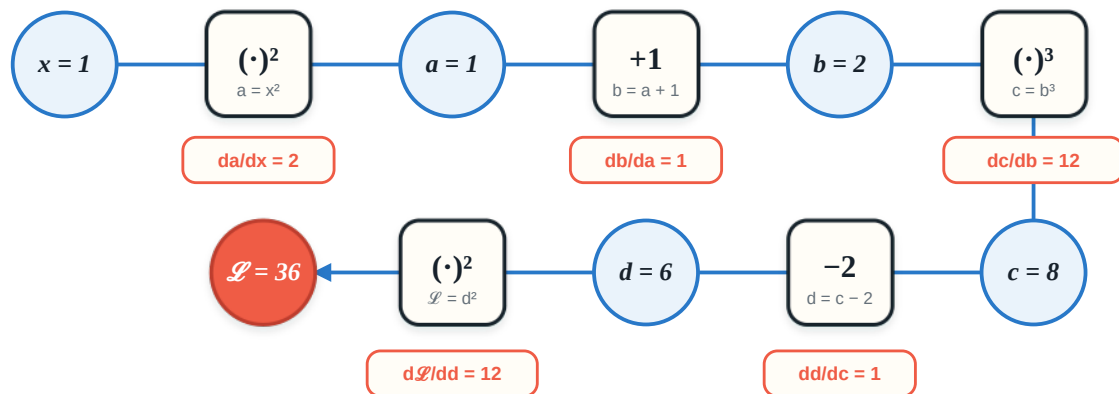
Figure 5: Every operation differentiates only its own input-output relationship.
