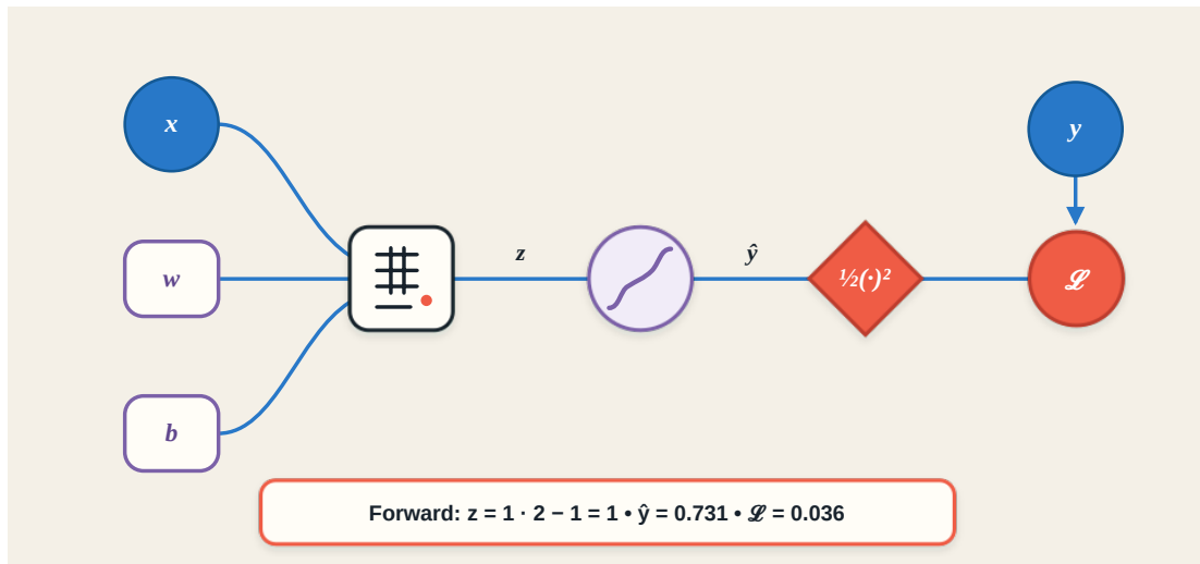
Figure 7: The completed sigmoid-neuron graph.
