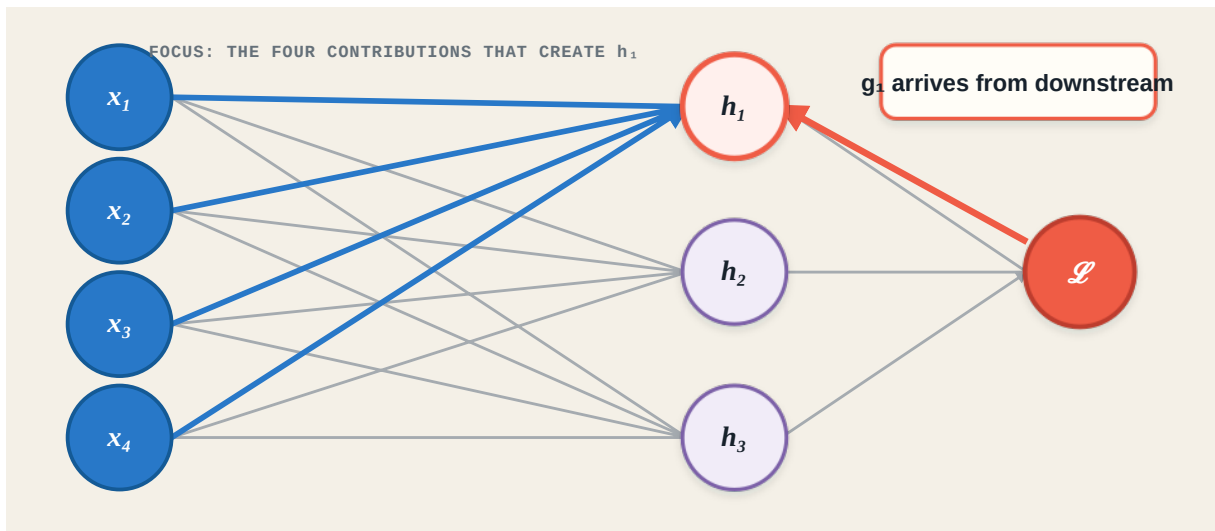
Figure 10: A four-to-three linear layer. The four edges that produce h_1 and the incoming message from the loss are highlighted.
