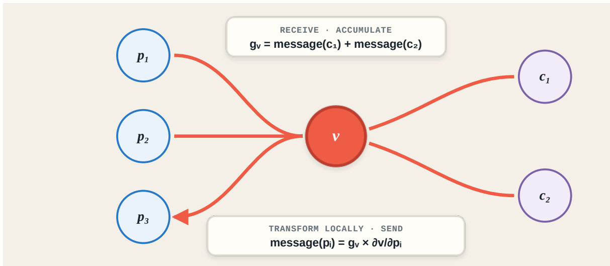
Figure 11: A node receives messages from its children, adds them, and sends locally transformed messages to its parents.
