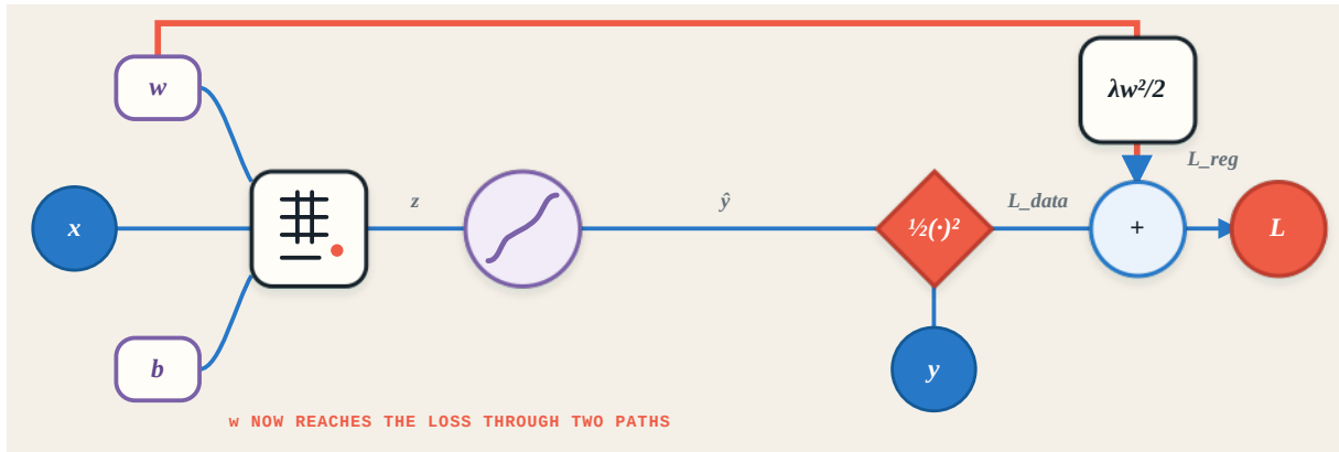
Figure 9: The weight w reaches the total loss through the data-loss path and the regularization path.
