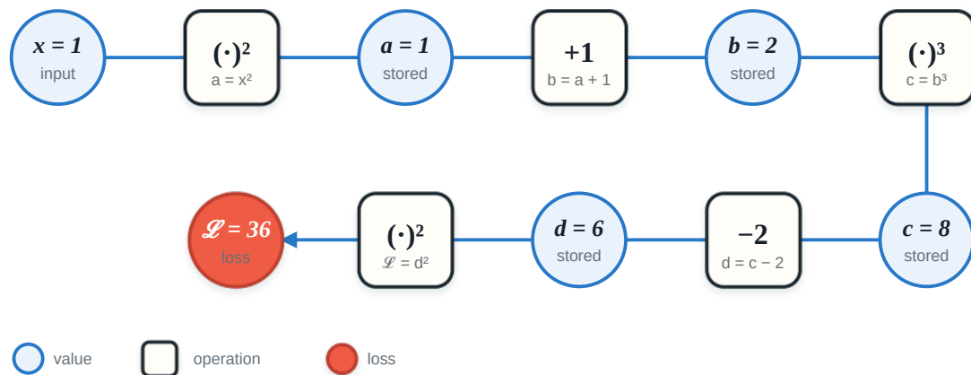
Figure 4: The forward graph evaluates the expression as five small operations and stores the intermediate values.
