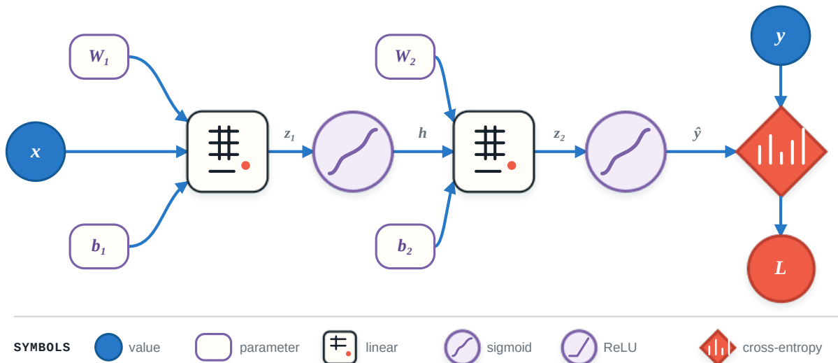
Figure 1: The symbolic computation graph used in the lecture: values are blue circles, parameters are purple rounded rectangles, affine maps are square blocks, sigmoid activations are purple circles, and binary cross-entropy is the coral loss node.
