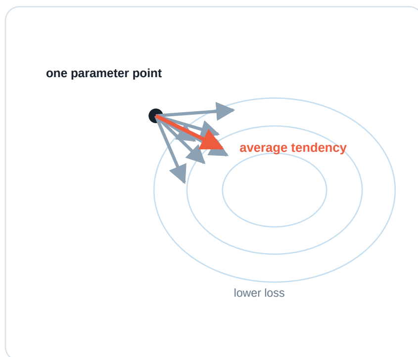
Figure 5: Several minibatches propose different negative-gradient update directions; their average follows the full-data tendency.
