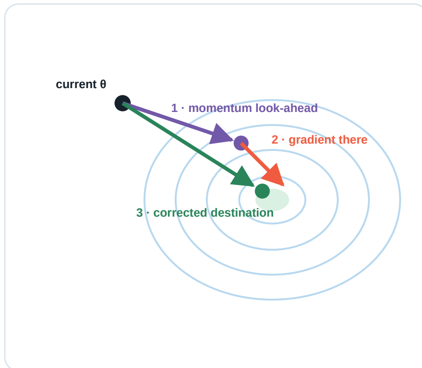
Figure 9: Nesterov follows momentum to a provisional point, measures the gradient there, and forms a corrected destination.
