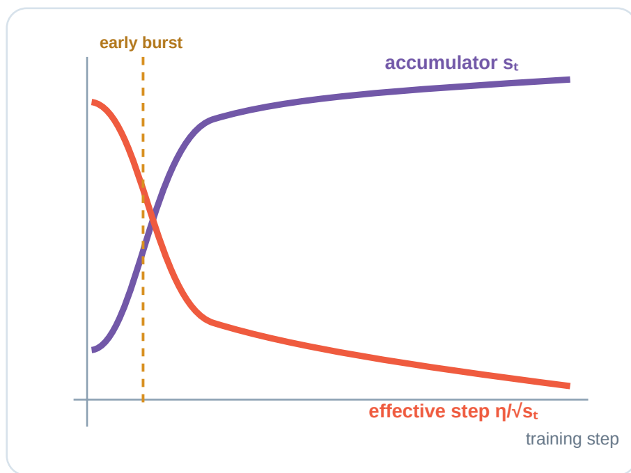
Figure 10: AdaGrad's accumulator rises while its effective learning rate shrinks after an early gradient burst.
