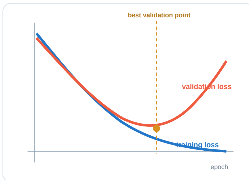
Figure 14: Training loss continues downward while validation loss turns upward after its best point.
