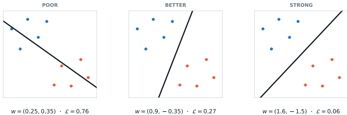
Figure 2: Three parameter settings produce three decision boundaries and three losses for the same data and model family.
