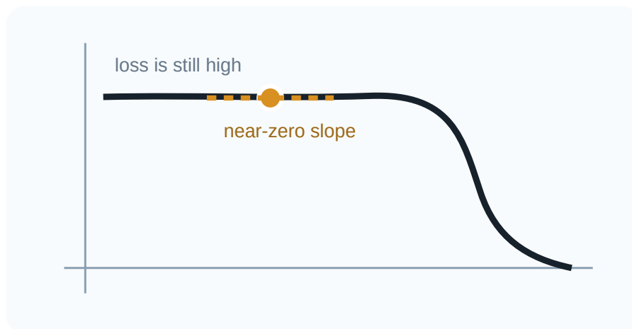
Figure 8: A near-zero gradient can also occur on a high plateau.
