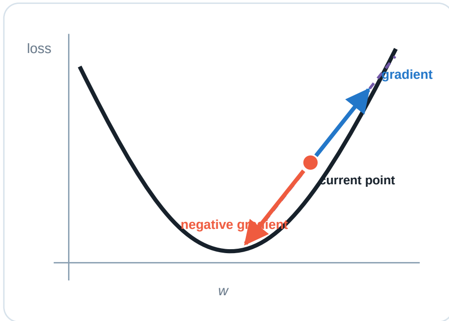
Figure 4: At the current point, the gradient follows the increasing tangent direction and the negative gradient points downhill.
