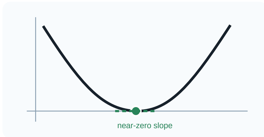
Figure 7: A near-zero gradient can occur at a low minimum.
