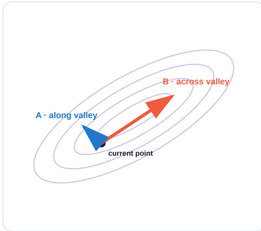
Figure 6: The long across-valley component dominates the small along-valley component.
