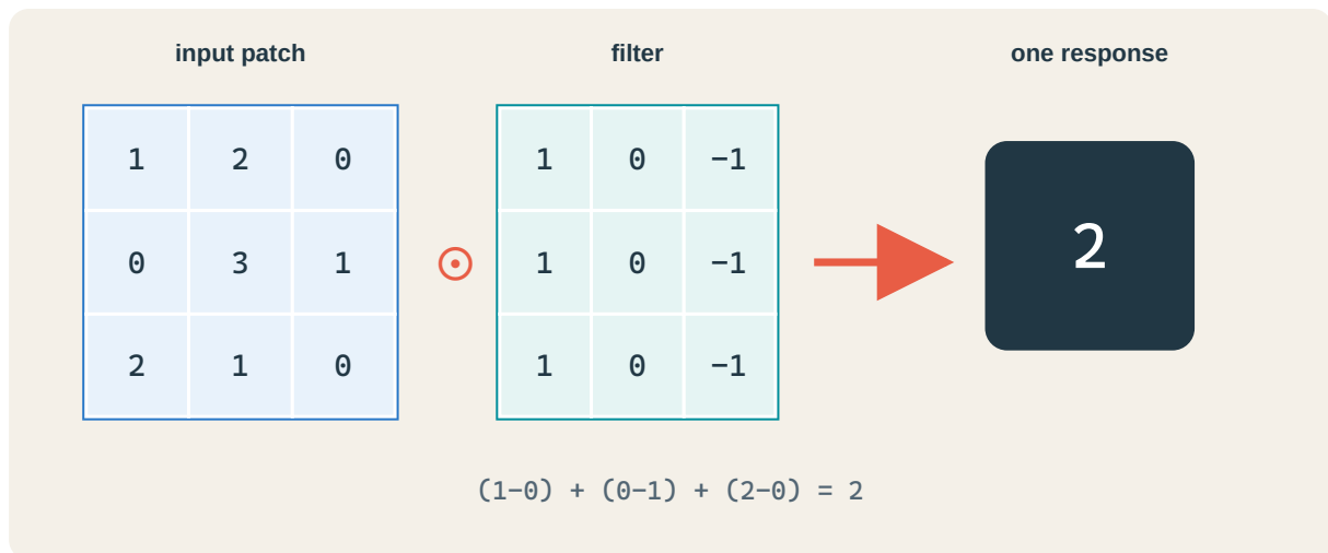
Figure 3: A 3 by 3 image patch and a vertical-change filter are multiplied elementwise and summed to produce the response 2. Original course SVG.
