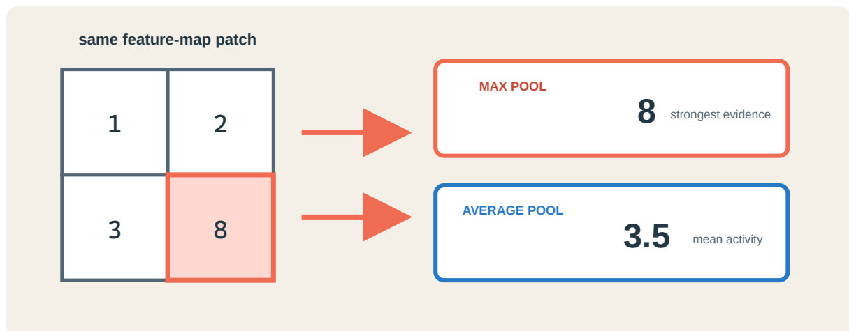
Figure 7: The same two-by-two patch produces 8 under max pooling and 3.5 under average pooling. Original course SVG.
