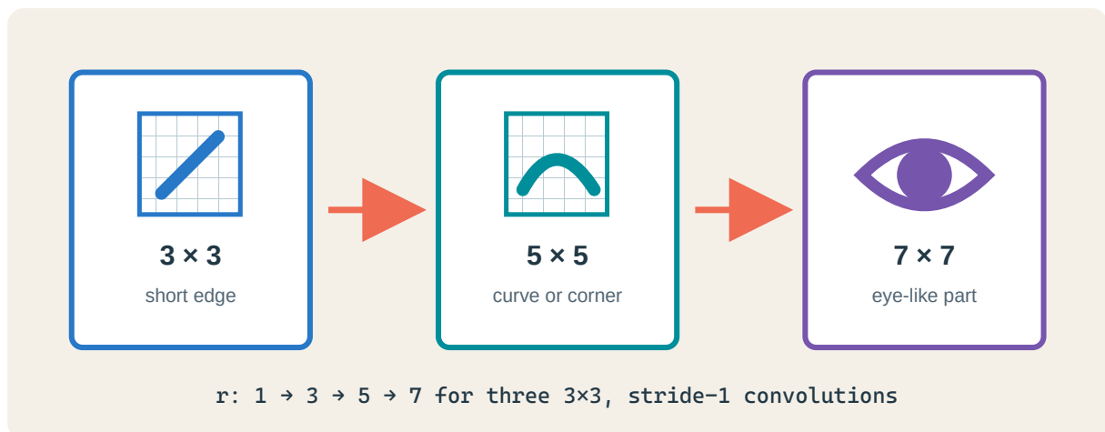
Figure 8: Three stride-one 3 by 3 convolutions expand the receptive field from 3 by 3 to 5 by 5 and then 7 by 7, enabling edge responses to be composed into motifs and an eye-like part. Original course SVG.
