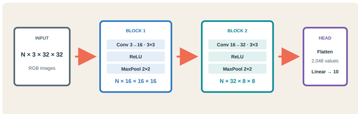
Figure 9: Tensor shapes through a two-block CNN: RGB input, two convolution-ReLU-pooling blocks, flattening, and ten output scores. Original course SVG.
