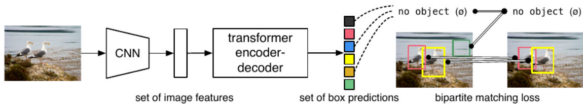
Figure 7: DETR maps an image through a CNN and transformer to a fixed set of predictions, then matches predictions uniquely to ground-truth objects. Source: Carion et al., Figure 1.
