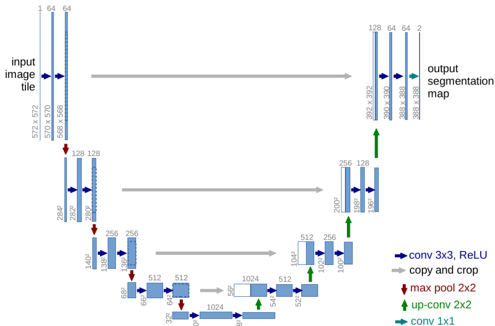
Figure 3: The original U-Net architecture has a contracting path, an expanding path, and copy-and-crop connections between matching resolutions. Source: Ronneberger et al., Figure 1.
