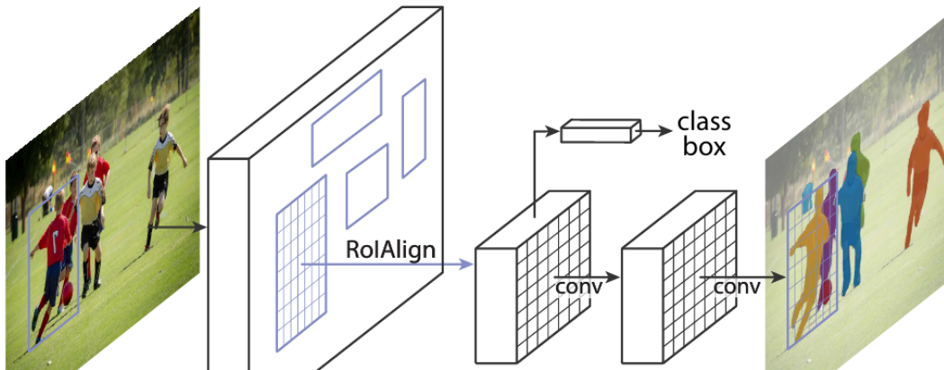
Figure 8: Mask R-CNN extends the Faster R-CNN region pipeline with a parallel fully convolutional mask branch. Source: He et al., Figure 1.
