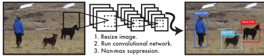
Figure 6: The original YOLO system resizes an image, runs one convolutional network, and applies non-maximum suppression. Source: Redmon et al., Figure 1.
