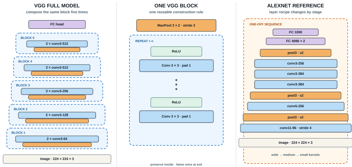
Figure 5: VGG represented as a full configuration, a reusable VGG block, and the AlexNet reference architecture. Original course SVG.
