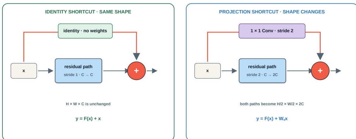
Figure 12: Identity and projection residual shortcuts compared side by side. Original course SVG.
