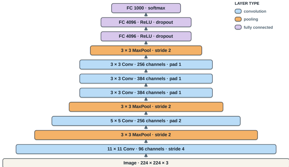
Figure 2: Course reconstruction of AlexNet as a sequence of compact layer bars. The diagram uses the visual grammar followed throughout this chapter.
