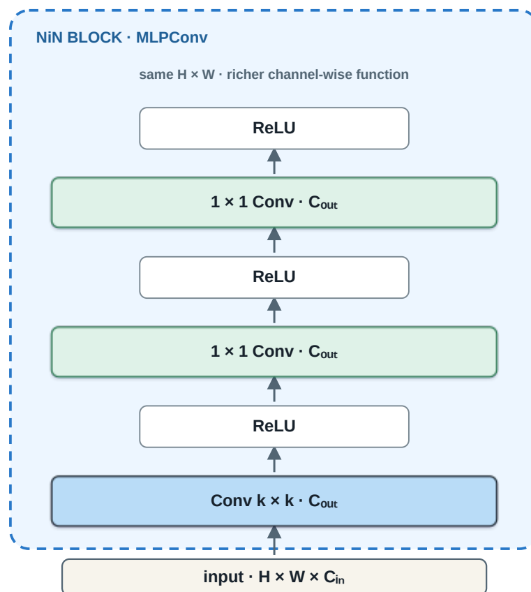
Figure 6: A NiN block begins with a spatial convolution and follows it with two one-by-one convolutional channel mixers. Original course SVG.
