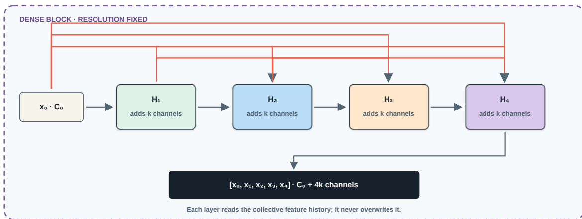
Figure 14: Four dense layers append new features to a shared feature history. Original course SVG.
