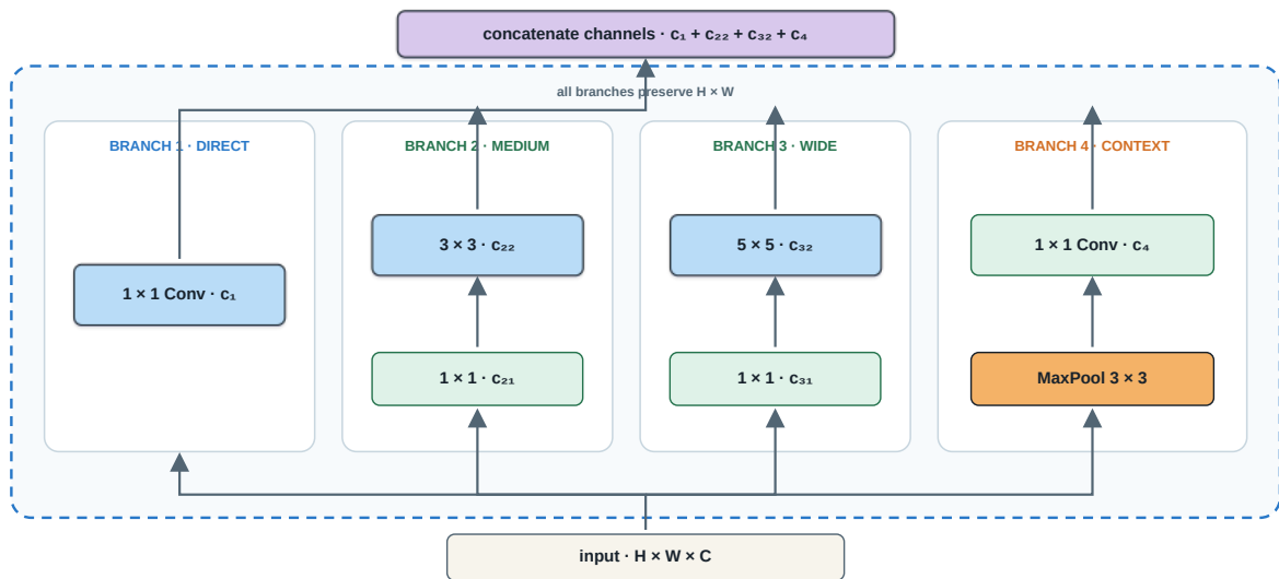
Figure 8: An Inception block with four parallel branches whose outputs are concatenated along channels. Original course SVG.
