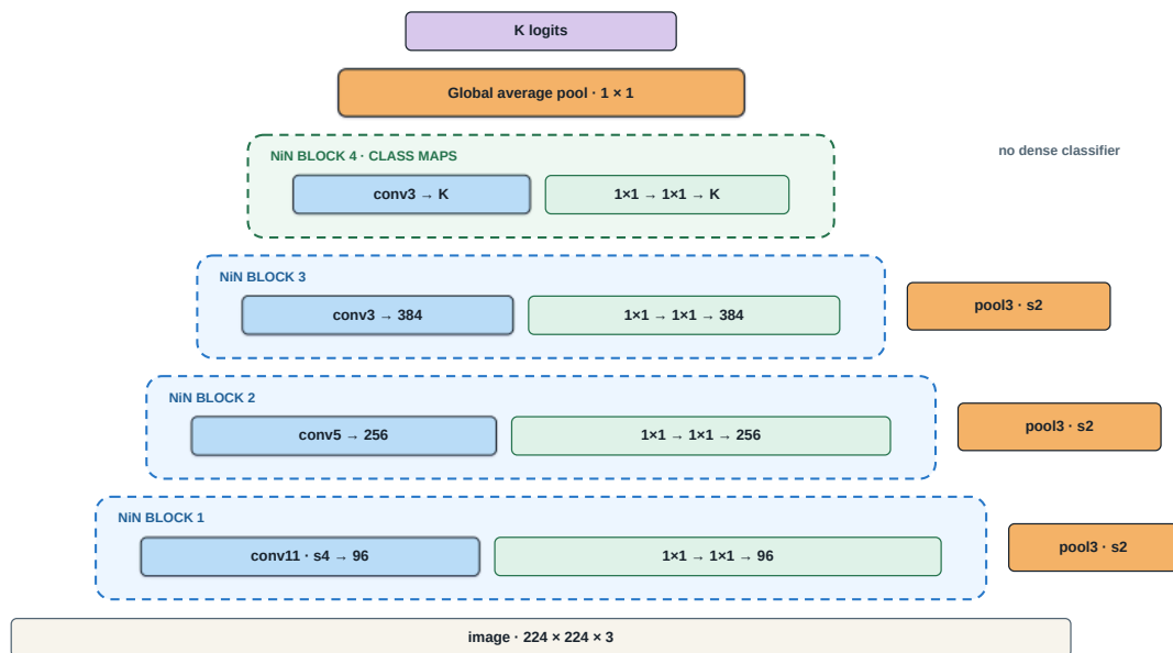
Figure 7: Full NiN architecture with four grouped NiN blocks and a global-average-pooling classifier. Original course SVG.
