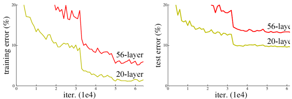
Figure 10: Training and test error curves for plain 20- and 56-layer networks. The deeper plain network performs worse. Source: He et al., Figure 1.
