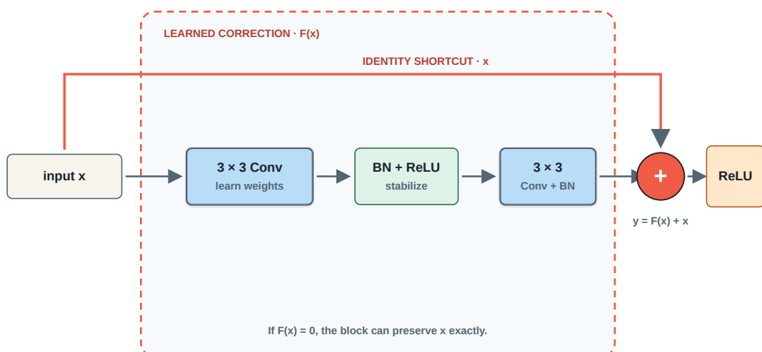
Figure 11: Residual block with a learned two-convolution path and an identity shortcut meeting at addition. Original course SVG.
