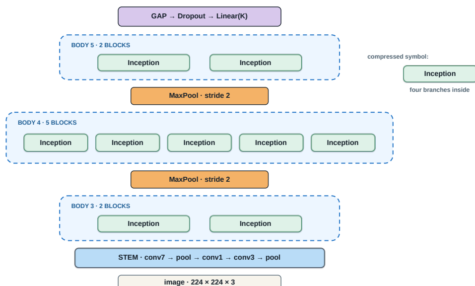
Figure 9: Compressed GoogLeNet architecture assembled from nine Inception modules. Original course SVG.
