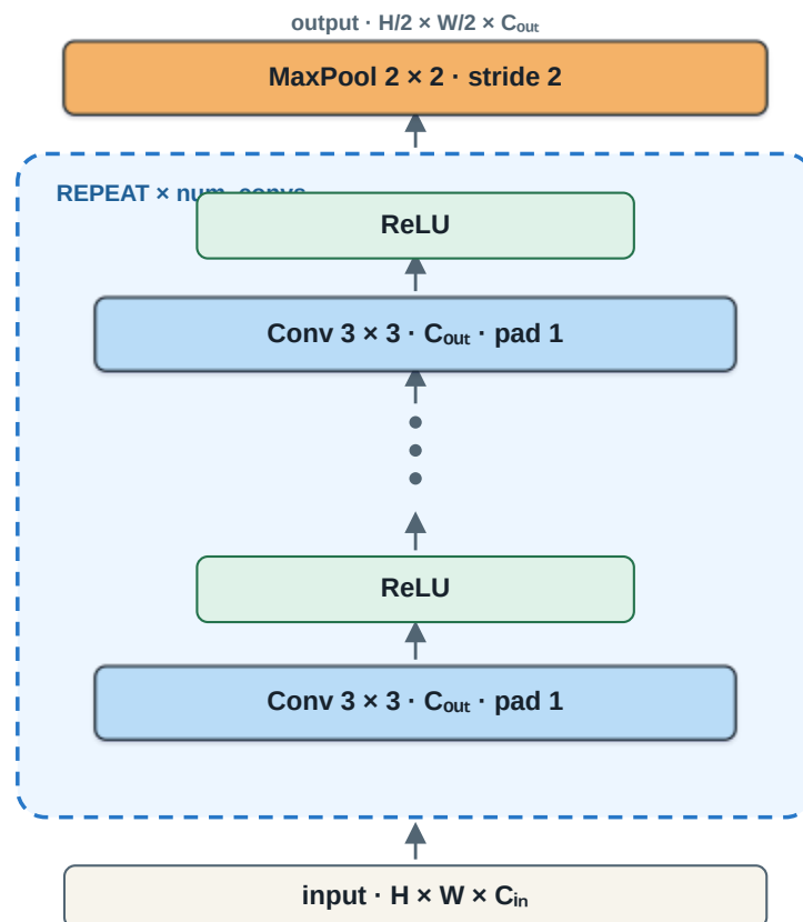
Figure 4: A VGG block groups repeated padded three-by-three convolutions and ReLU operations before one max-pooling step. Original course SVG.
