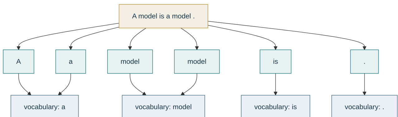
Figure 2: Repeated token instances point to the same vocabulary entry.
