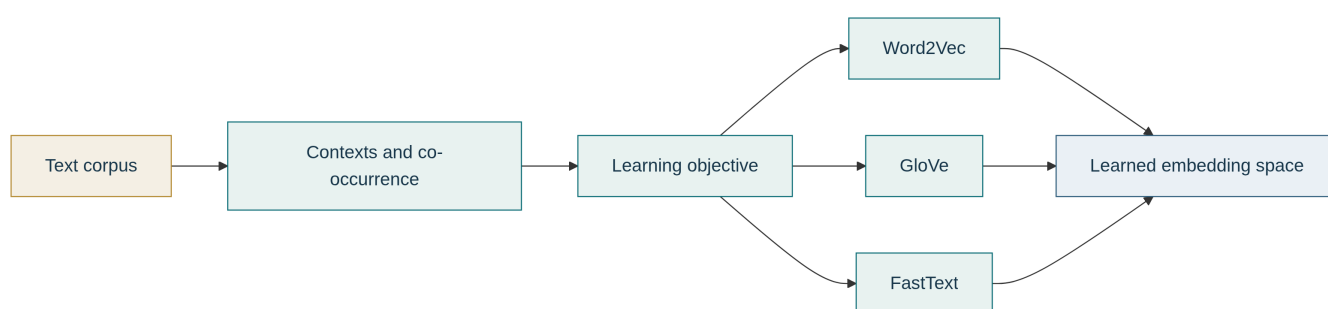
Figure 10: Chapter 3 moves from inspecting embeddings to learning them from patterns of context.
