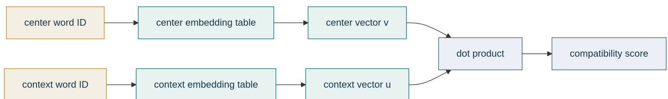
Figure 3: Skip-gram looks up a center vector and scores it against a context vector.
