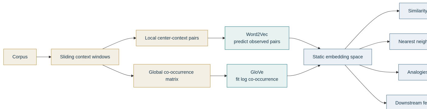
Figure 5: Two influential objectives turn the same distributional evidence into dense static vectors.
