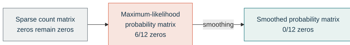
Figure 10: The observations do not change. Only the estimated probability table becomes dense.
