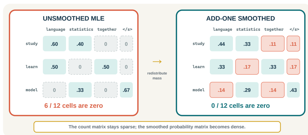
Figure 9: Smoothing redistributes probability mass from observed transitions to formerly zero cells.
