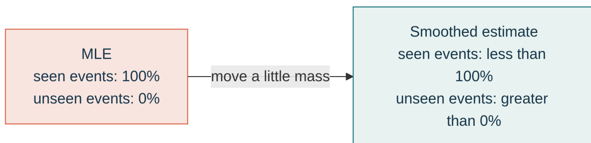
Figure 8: Smoothing does not create new observations; it redistributes estimated probability mass.
