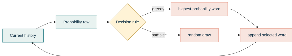
Figure 6: Autoregressive generation repeatedly selects a word, appends it, and treats the result as the next history.
