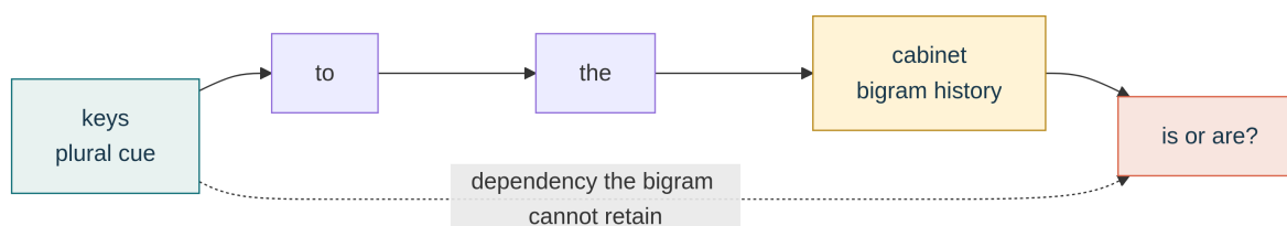
Figure 12: The predictive cue can lie outside a fixed n-gram window.
