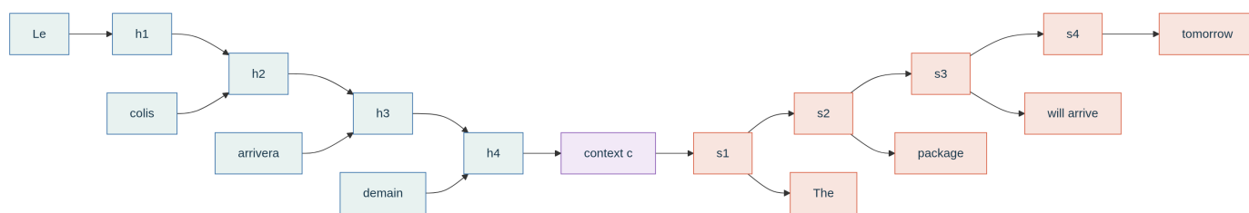
Figure 8: The final encoder state initializes a decoder that generates a new sequence. Encoder and decoder may have separate parameters.
