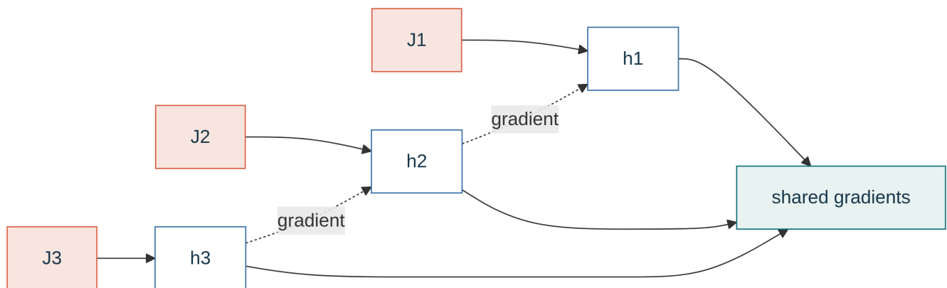
Figure 6: Each time step uses the same parameters, so its local contribution is added to one shared parameter gradient.
