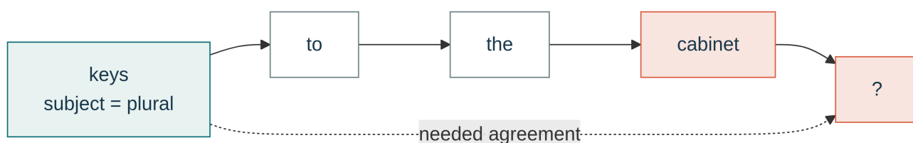
Figure 3: The sentence contains the needed feature, but the bigram representation exposes only the final token to the predictor.
