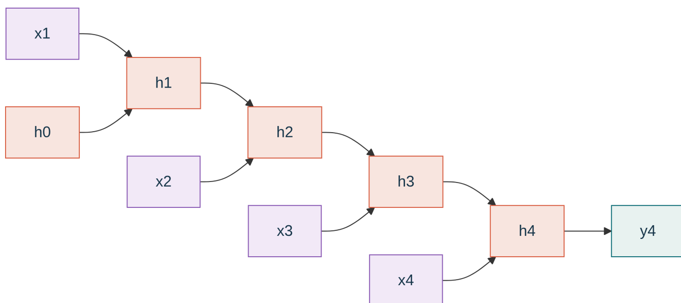
Figure 5: Unfolding reveals repeated applications of one state-update rule. The graph grows with the sequence, but the parameter set does not.
