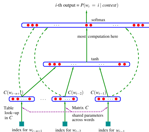
Figure 4: The neural probabilistic language-model architecture. Reproduced from Bengio et al. (2003), Fig. 1.
