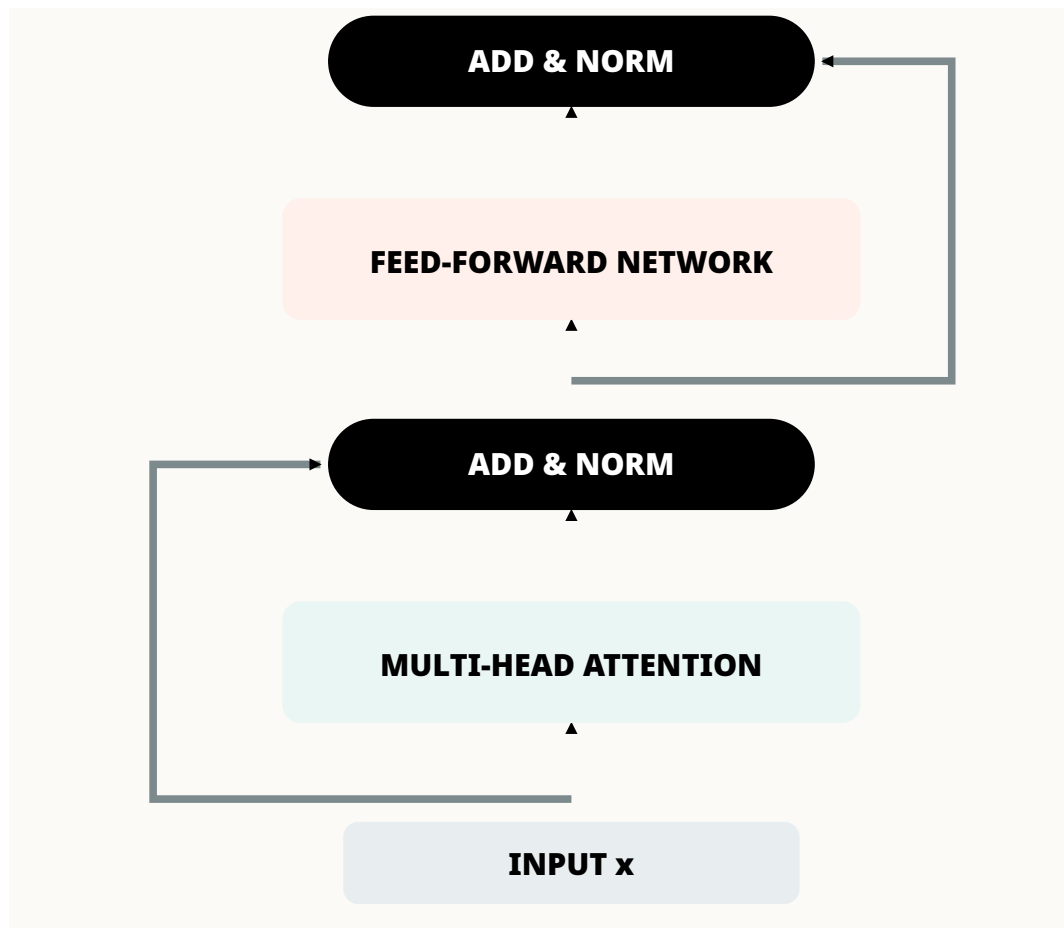
Figure 6: The classical post-norm block used in the lecture: each learned sublayer has a residual route followed by Add & Norm.
