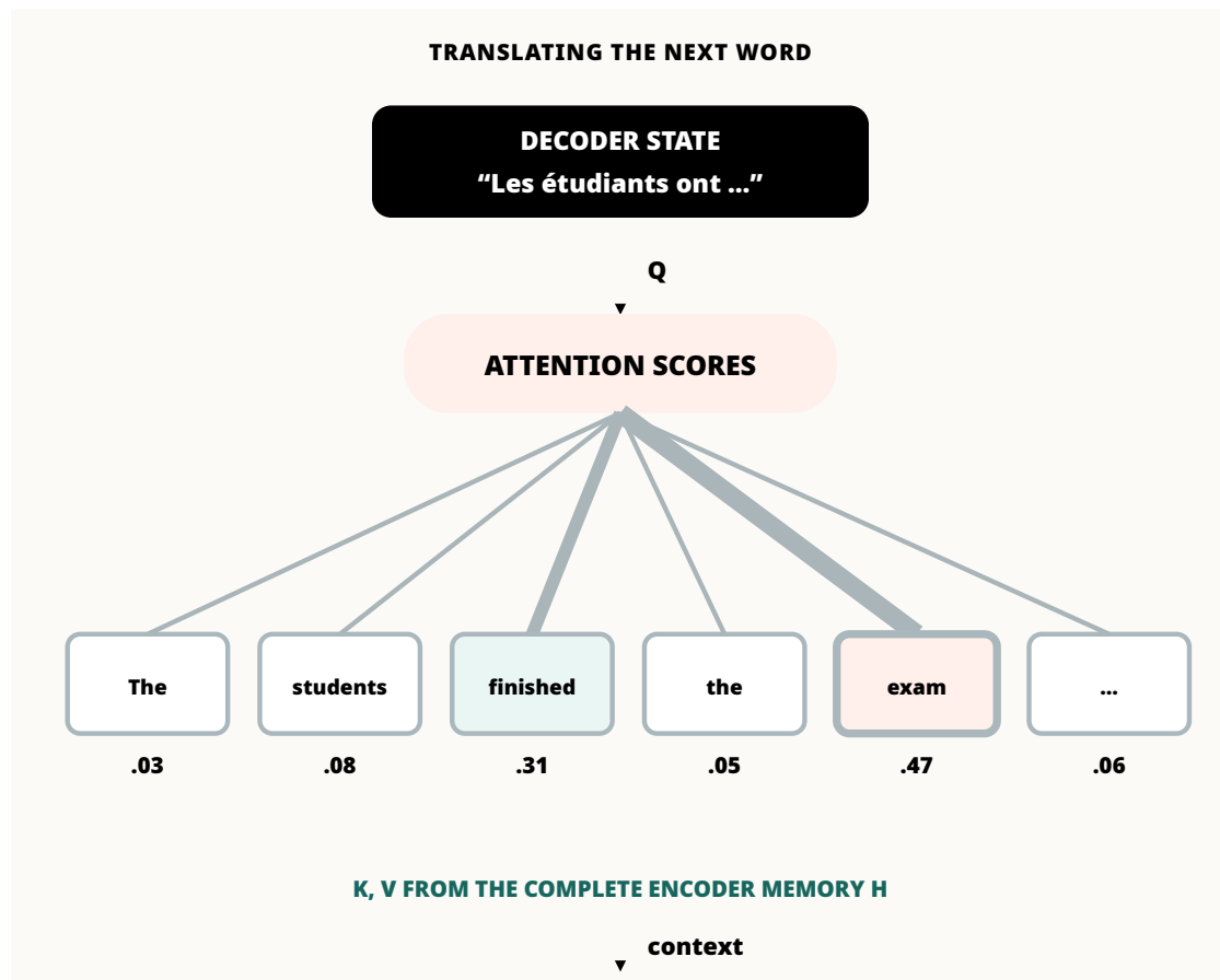
Figure 9: Cross-attention keeps the origins inspectable: the decoder supplies the query while the complete encoder memory supplies keys and values.
