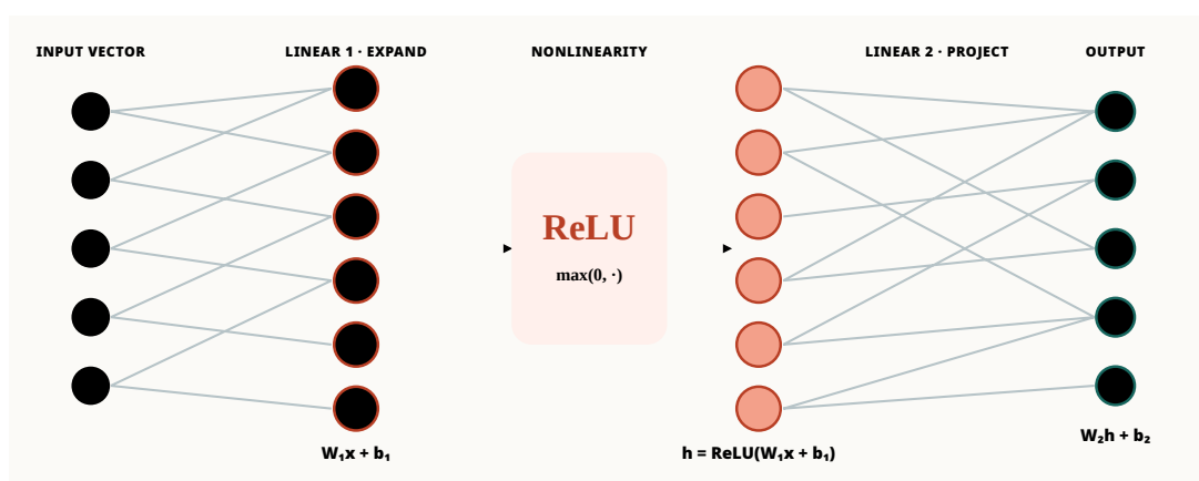
Figure 4: The lecture’s neural-network view of the position-wise FFN: a first affine layer, ReLU, and a second affine layer return each token to the model dimension.
