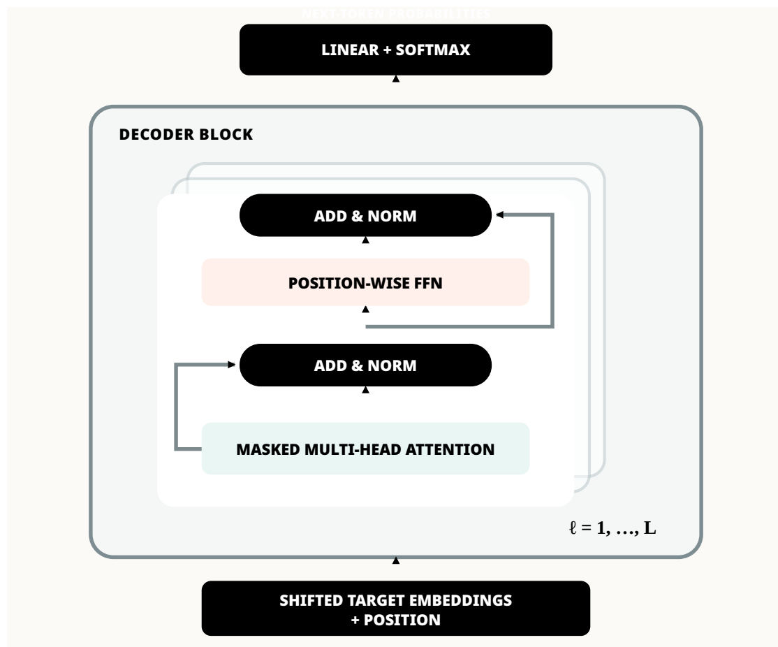
Figure 7: A decoder is a stack of repeated decoder blocks. Masked self-attention, residual normalization, and the FFN repeat before the final Linear + Softmax head.
