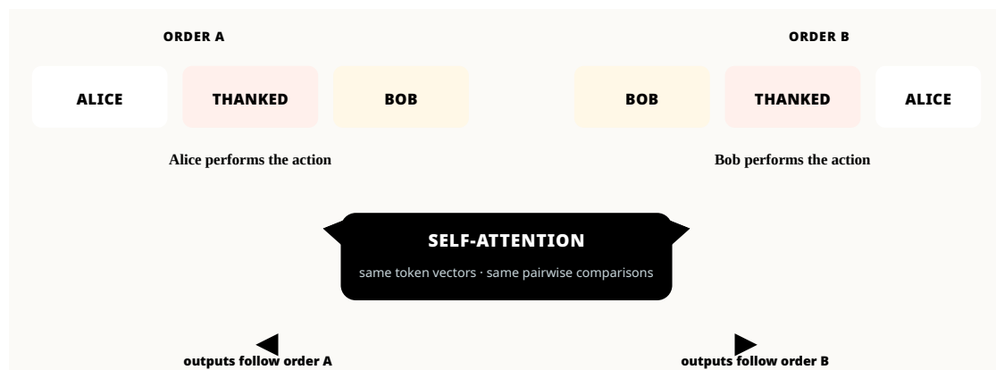
Figure 2: Without a position signal, self-attention follows a permutation but cannot identify the changed order. This standalone vector figure is generated from the lecture’s original SVG code.
