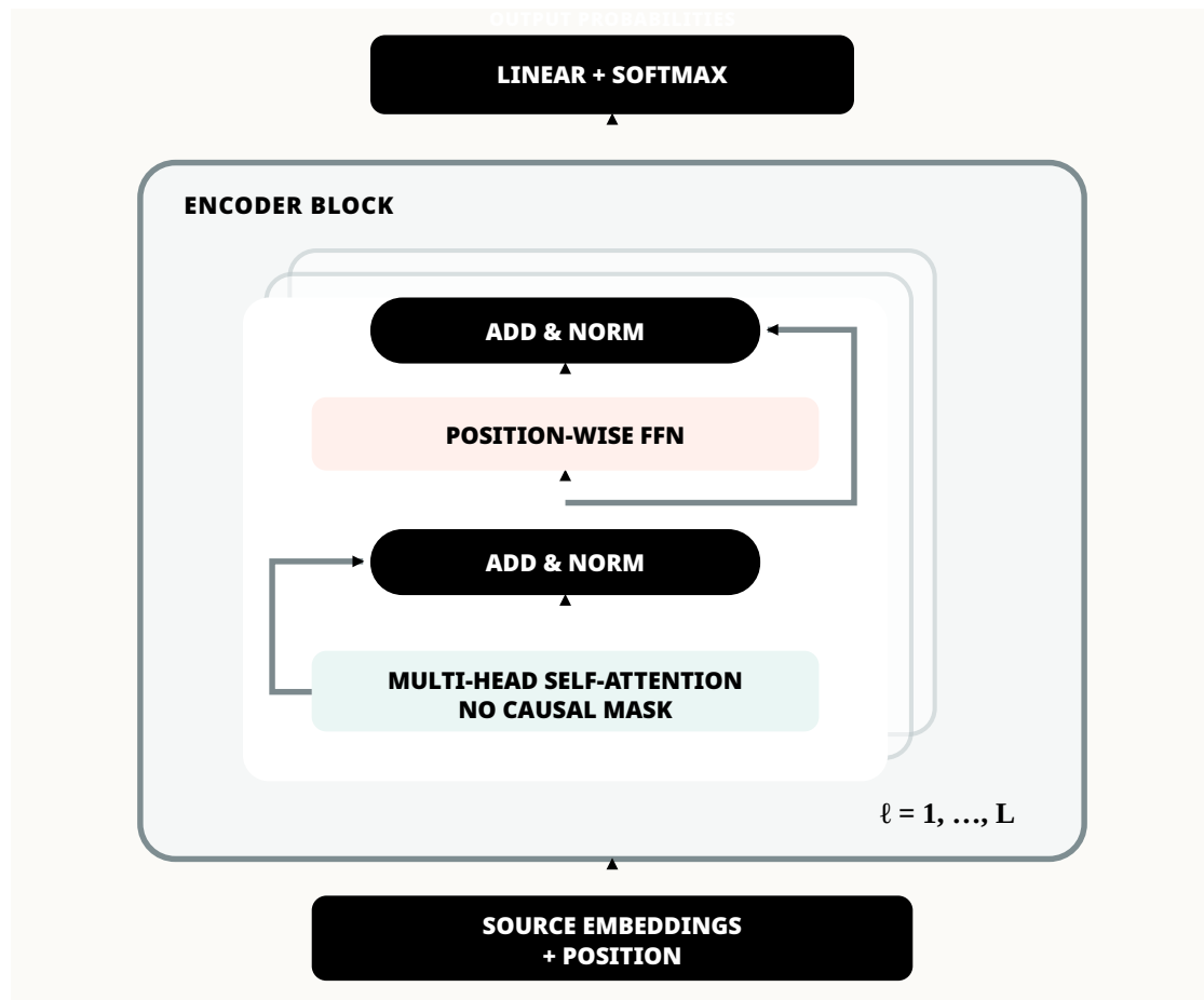
Figure 8: The corresponding encoder stack uses the same repeated-block visual language but removes the causal mask, allowing full source context.
