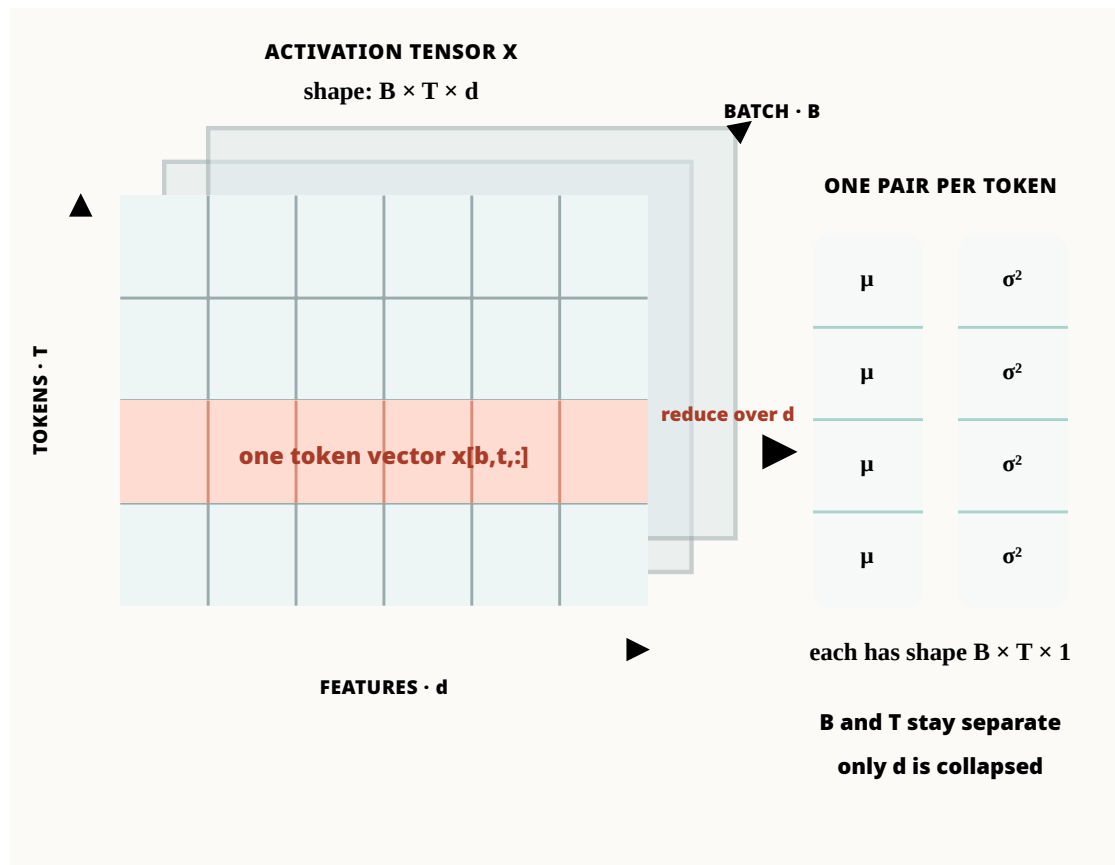
Figure 5: LayerNorm operates along the feature dimension of each token representation; it does not aggregate across tokens or batches.
